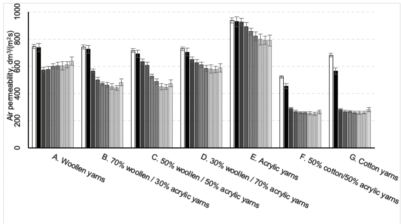
Figure 7. Air permeability of tested knitted fabrics before wet treatment, after antimicrobial treatment, and after repeated washing and drying.
