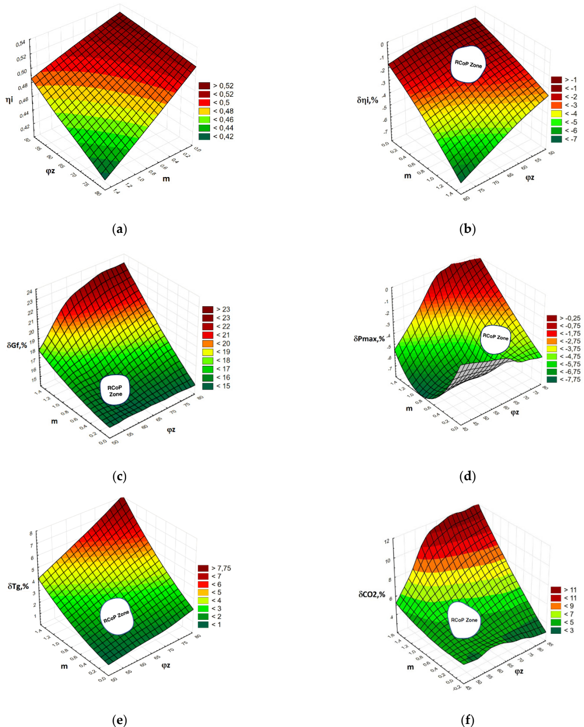
Figure 7. A relative change in engine operational parameters when switching from diesel fuel to microalgae oil: (a) Indicated efficiency of an engine fueled by diesel fuel; (b) Indicated efficiency (change); (c) Hourly fuel consumption; (d) Maximum cycle pressure (combustion pressure); (e) Exhaust gas temperature; (f) \text{CO}_2 emissions; RCoP Zone—the zone of rational combination of m and \varphi_z parameters).
