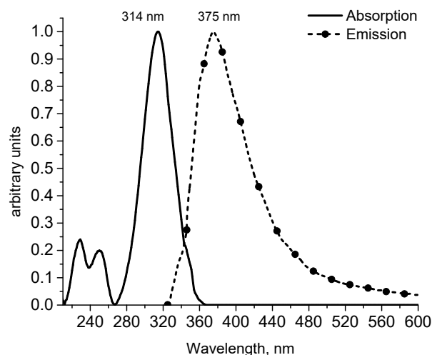
Figure 4. Absorption and emission ( \lambda_{\text{ex}} = 320 nm) spectrum of compound 4 in THF.
