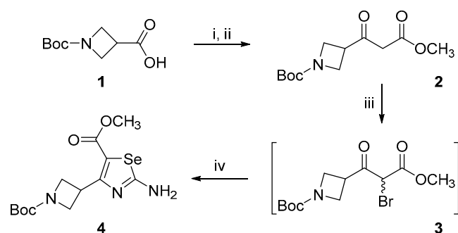
Scheme 1. Synthesis of methyl 2-amino-4-[1-( tert -butoxycarbonyl)azetidin-3-yl]-1,3-selenazole-5-carboxylate ( 4 ). Reagents and conditions: (i) Meldrum's acid, DMAP, EDC, DCM, r.t., 18 h; (ii) MeOH, 60 °C, 18 h; (iii) NBS, ACN, r.t., 2 h; (iv) selenourea, MeOH, r.t., 2 h.
