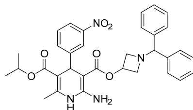
Figure 2. Structure of azelnidipine.
