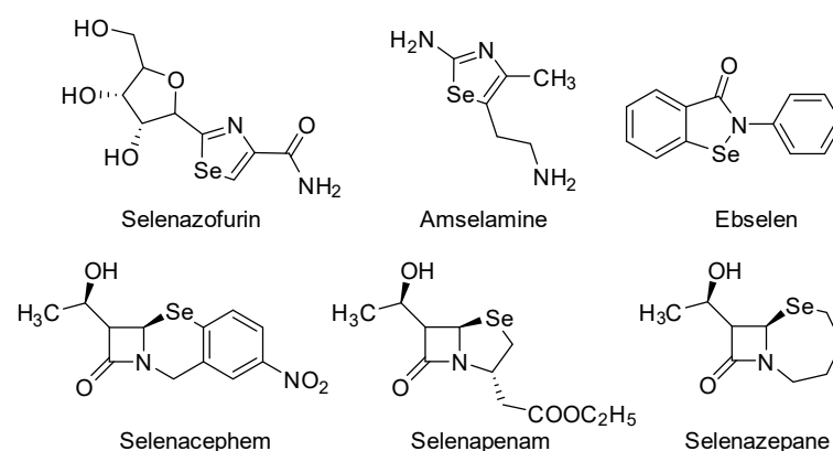
Figure 1. Biologically active organoselenium compounds.
