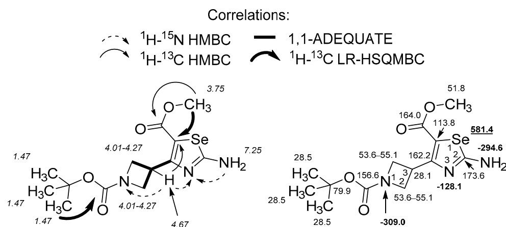
Figure 3. Relevant 1,1-ADEQUATE, ^1\text{H} - ^{13}\text{C} HMBC, ^1\text{H} - ^{15}\text{N} HMBC, ^1\text{H} - ^{13}\text{C} LR-HSQMBC correlations and ^1\text{H} NMR (in italics), ^{15}\text{N} NMR (in bold), ^{77}\text{Se} (in bold, underlined) and ^{13}\text{C} -NMR chemical shifts of compound 4 .
