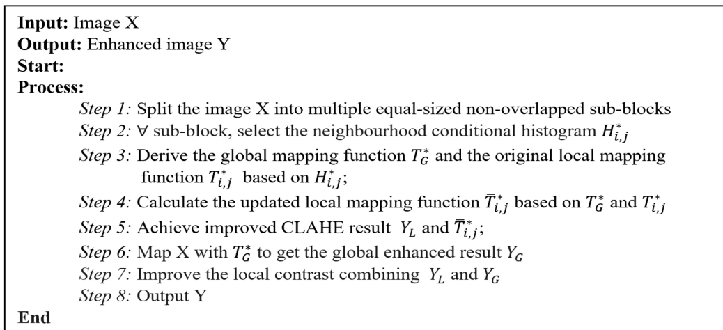
Figure 3. Algorithm of image enhancement.
