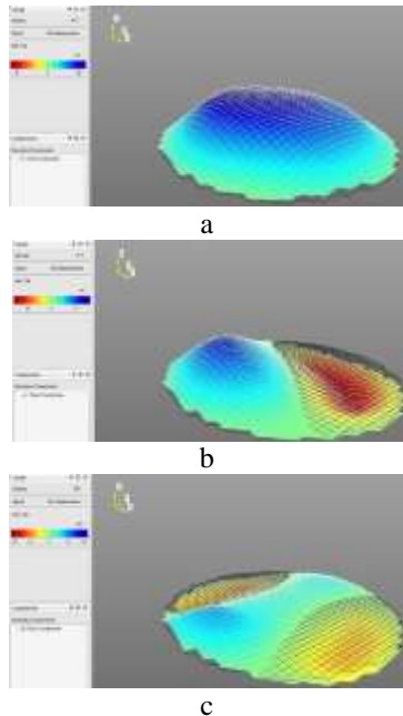
Fig. 5 Experimental shapes of the surface of membrane with piezoelectric element Sonox P502: a) frequency 2.85 kHz; b) frequency 5.22 kHz; c) frequency 15.77 kHz
