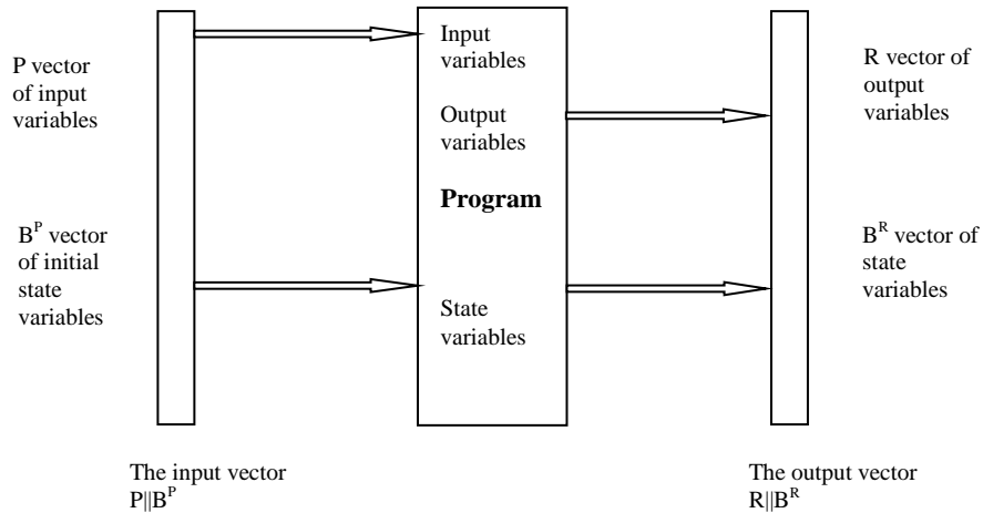
Fig. 2. Interconnecting of program variables with the input and output vectors
