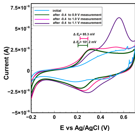
Figure 7. Cyclic voltammograms of [\text{Fe}(\text{CN})_6]^{3-/4-} for LT via changing potential window interval.
