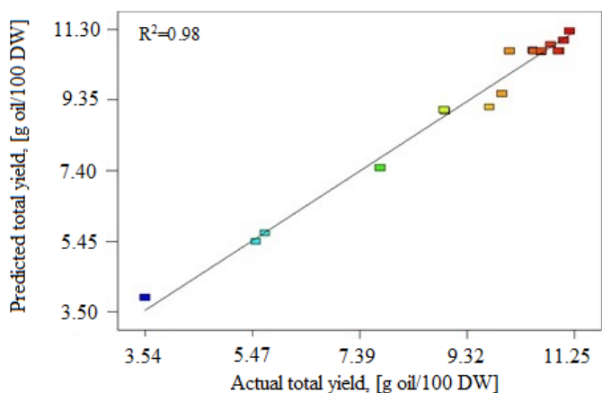
Figure 3.1. Comparison of the actual and predicted values for the lipophilic extract yield in SFE
