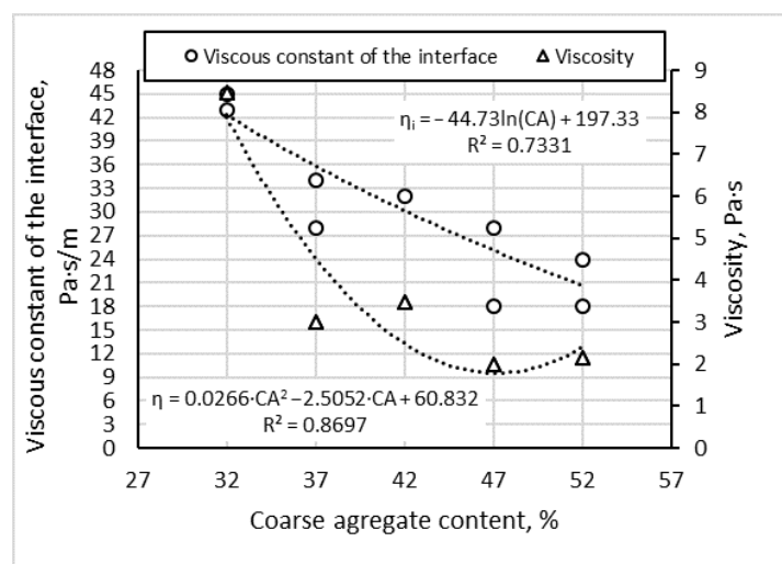
Figure 7. Relationship between the viscous constant of the interface and the viscosity of concrete, when the CA content in the AM changes from 32 to 52%.
