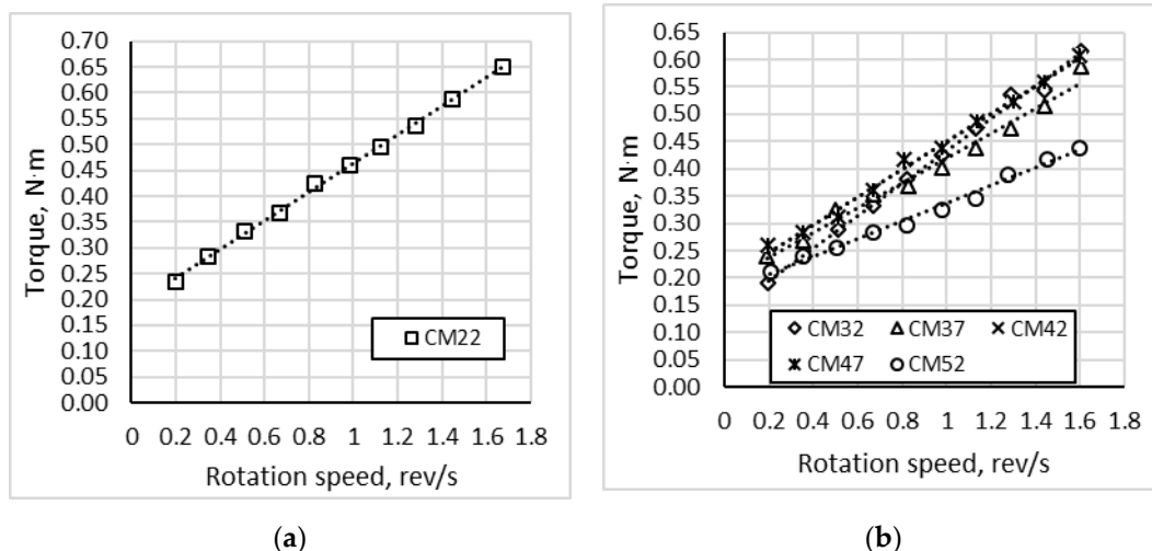
Figure 3. Evolution of the torque with the rotation speed while the CA content in the AM changes from 22 to 52%: (a) partial shearing of the concrete, (b) shearing was localised at the concrete steel interface.
