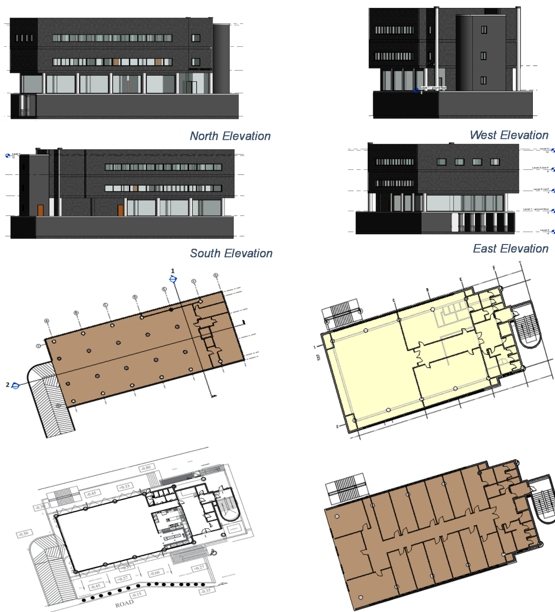
Figure 2. Building Sections and Plan Views—Frederick University, Nicosia Campus.
