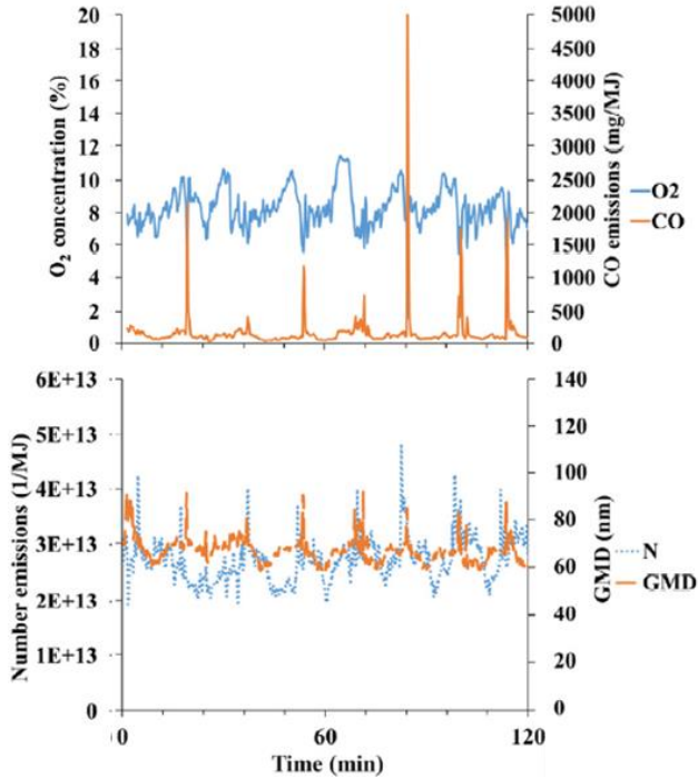
Fig. 1 Time series of O 2 , CO, particle number emissions and particle number mean diameters during combustion of bark pellets [10]
