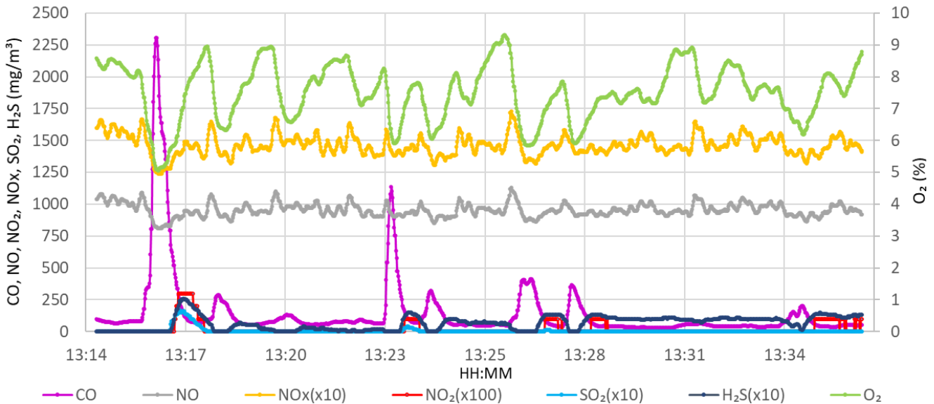
Fig. 5 Experimental boiler model emissions during combustion of wood pellets
