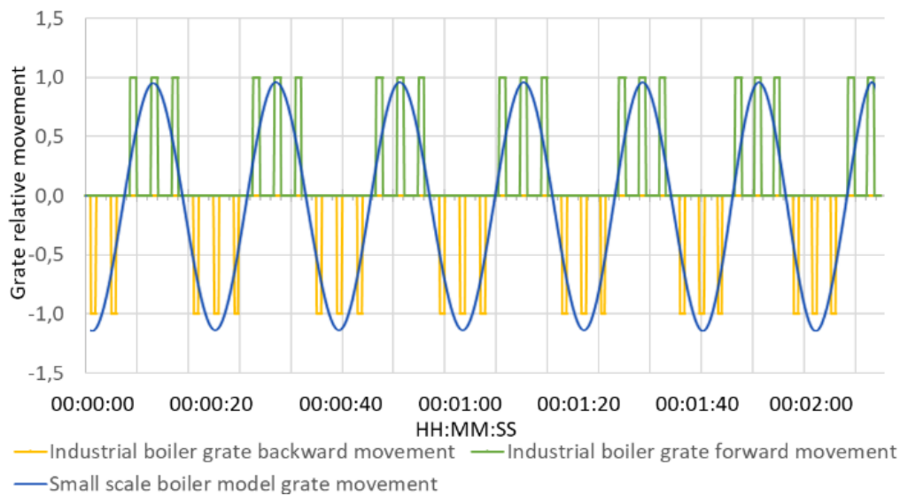
Fig. 7 Industrial and experimental boiler model grate motion characteristics
