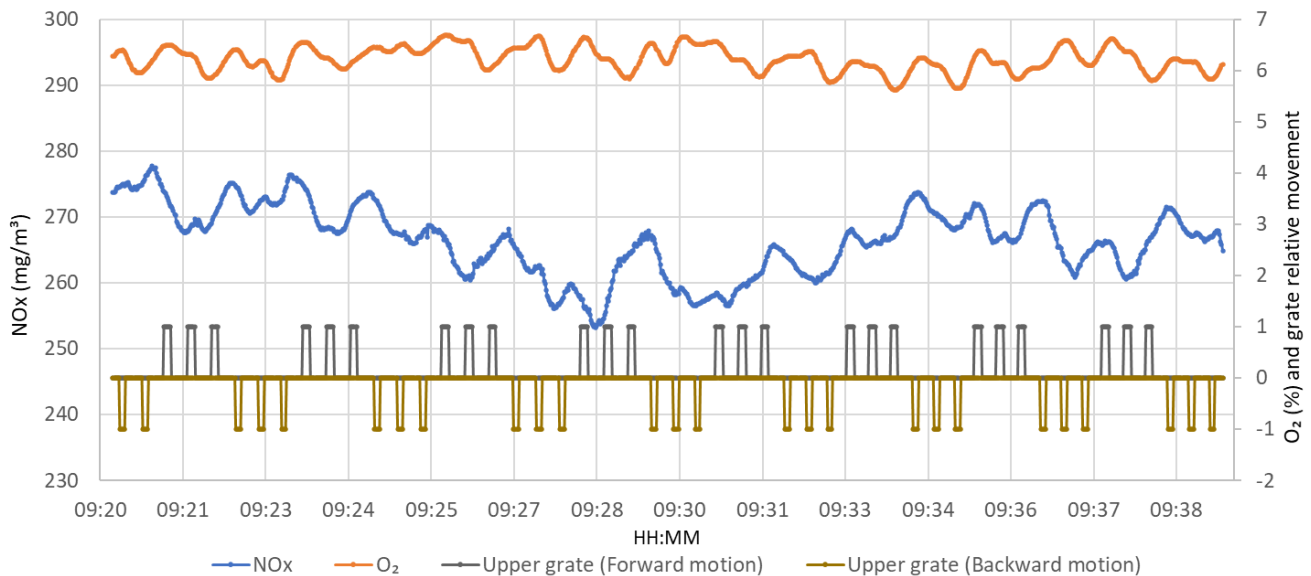
Fig. 8 The dependence of the 4 MW boiler flue gas emissions on the movement characteristics of the reciprocating grate
