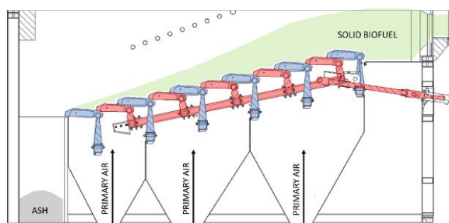
Fig. 3 A simplified schematic view of reciprocating grate
