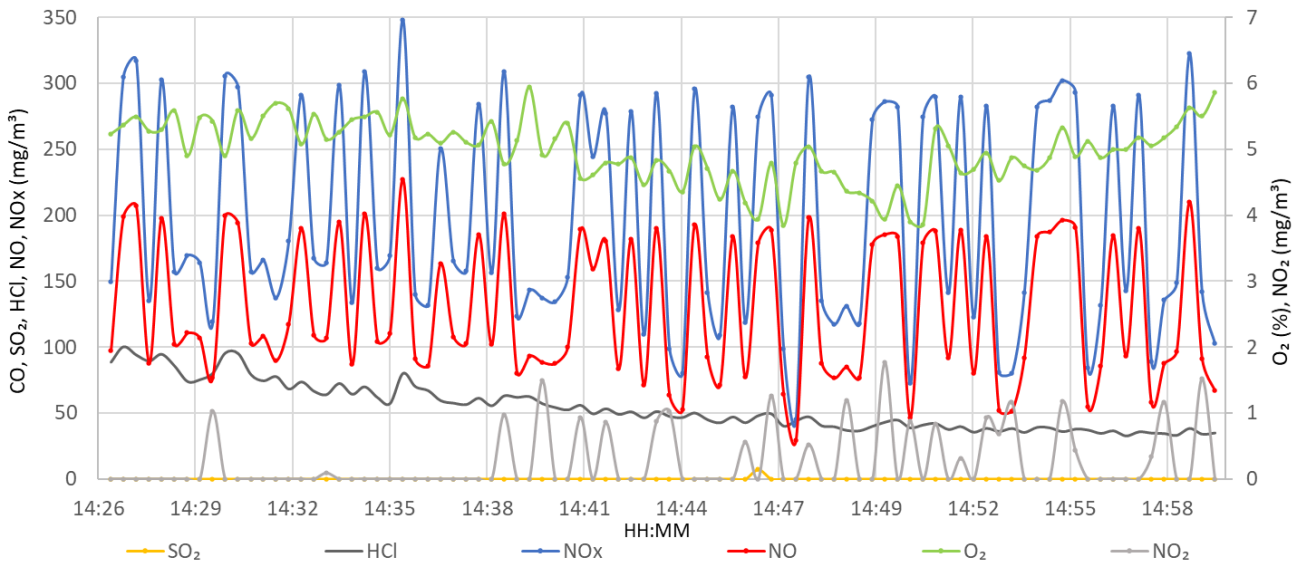
Fig. 4 8 MW boiler pollutant concentrations in combustion products
