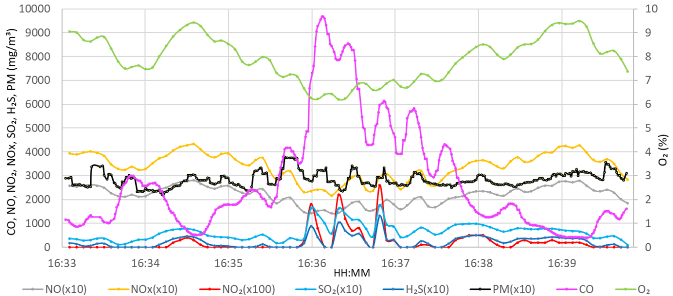
Fig. 6 Experimental boiler model emissions concentrations during combustion of sunflower pellets
