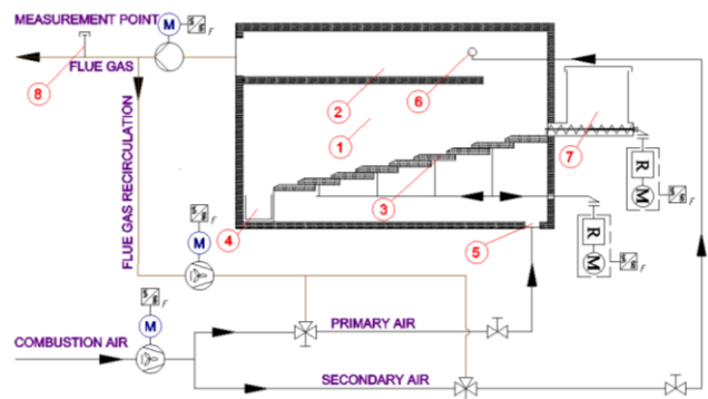
Fig. 2 A simplified schematic view of industrial and experimental model of biofuel boilers: 1 – primary combustion zone; 2 – secondary combustion zone; 3 – reciprocating grate; 4 – ash pit; 5 – supply of the primary air; 6 – supply of secondary air; 7 – supply of solid biofuel; 8 – gaseous emissions and particulate matter measurement point
