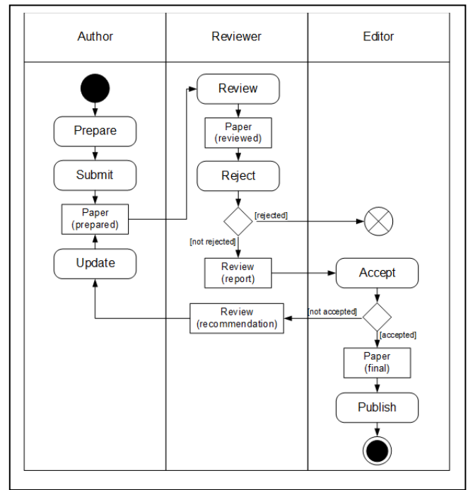
Fig. 4. Full UML Activity model generated from Enterprise model of an example of Paper submission for publishing process
