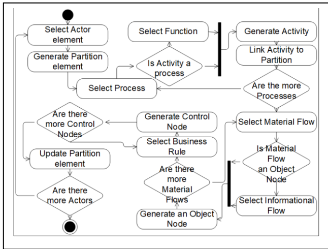
Fig. 3. UML Activity Model transformation algorithm [19][20]
