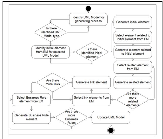
Fig. 2. The top level transformation algorithm of UML models generation from EM process [19][20]
