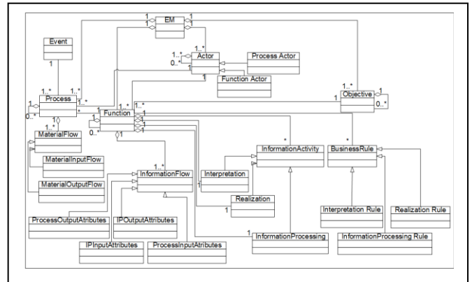
Fig. 1. EMM class diagram [6][7][8]
