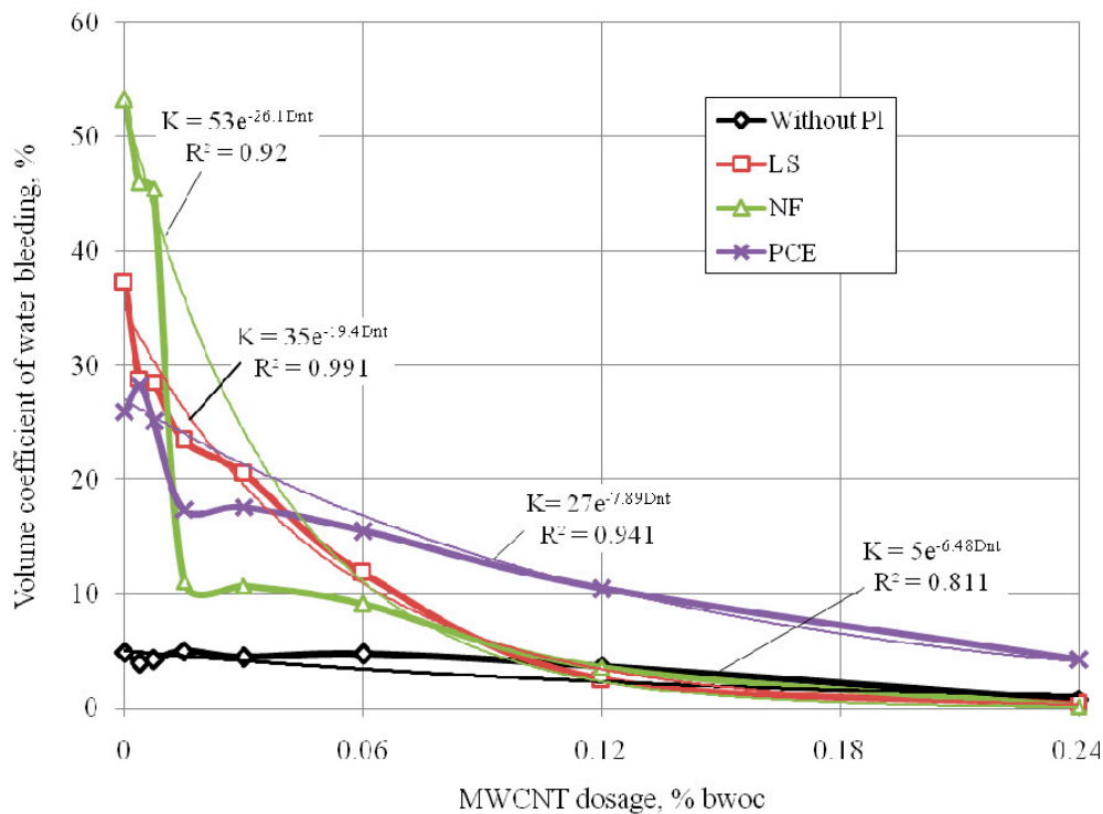
Figure 17. Water bleeding of nanomodified cement pastes with and without PI.
