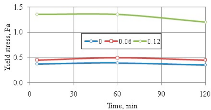
Figure 14. Yield stress of nanommodified cement paste with PCE 5, 60, and 120 min after cement paste mixing.
