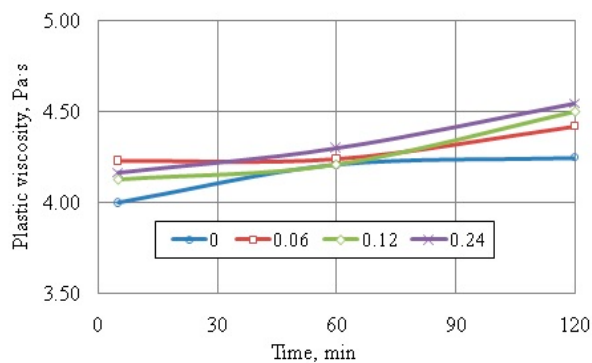
Figure 15. Plastic viscosity of nanommodified cement paste without PI 5, 60, and 120 min after cement paste mixing.
