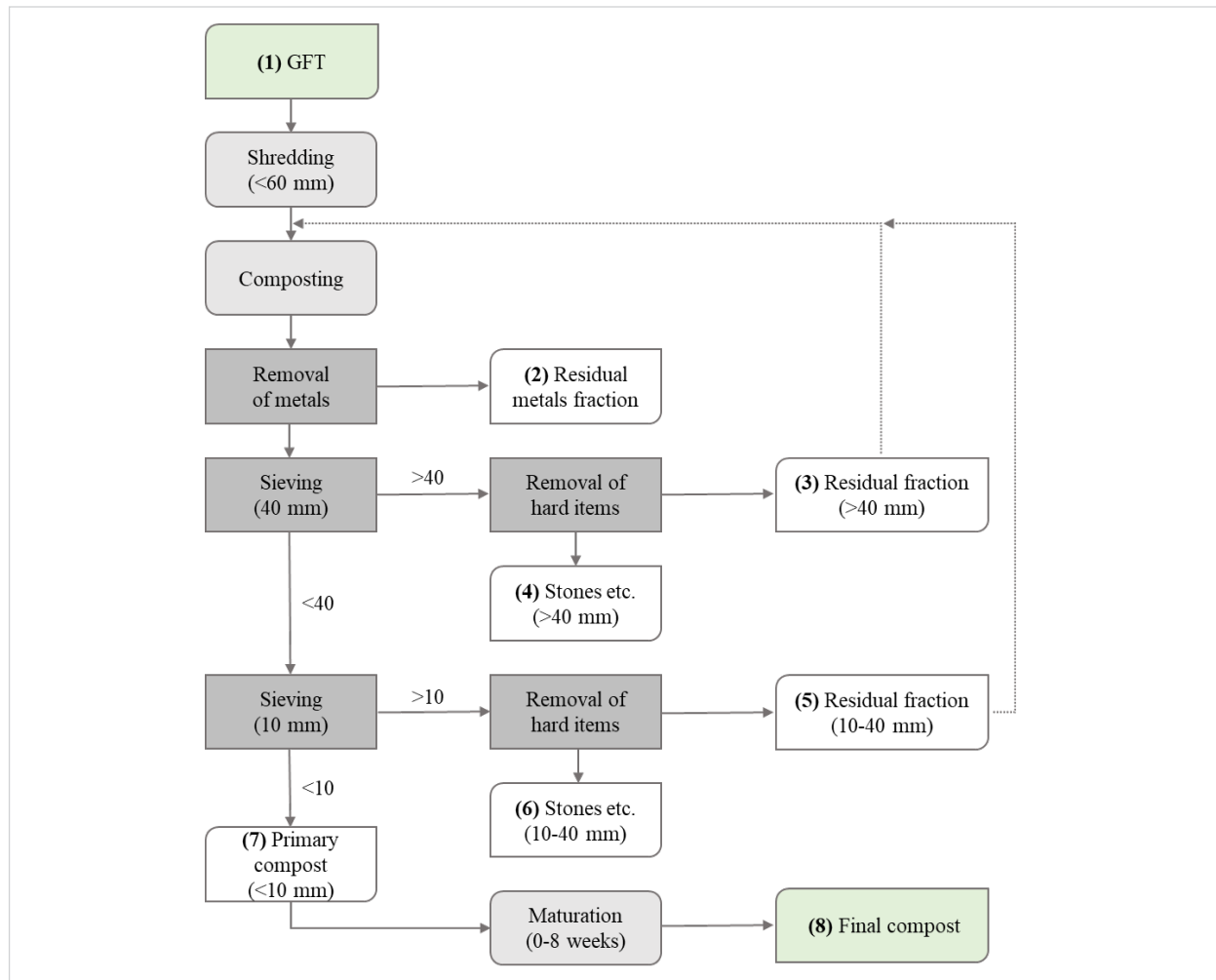
Fig. 3. A schematic presentation of the organic waste treatment process at the Van Kaathoven (Valor) facility, location Sint-Oedenrode. Dashed arrows indicate that the residual fractions (3) and (5) are occasionally (but not always) recirculated. Source: (Van der Zee and Molenveld, 2020)
