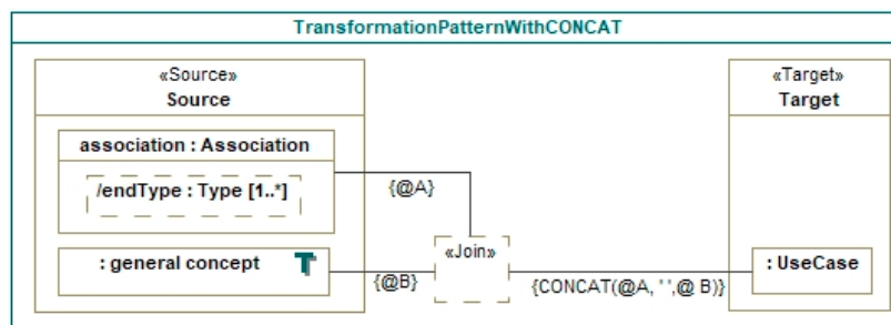
Figure 5. Sample transformation pattern with CONCAT() .
