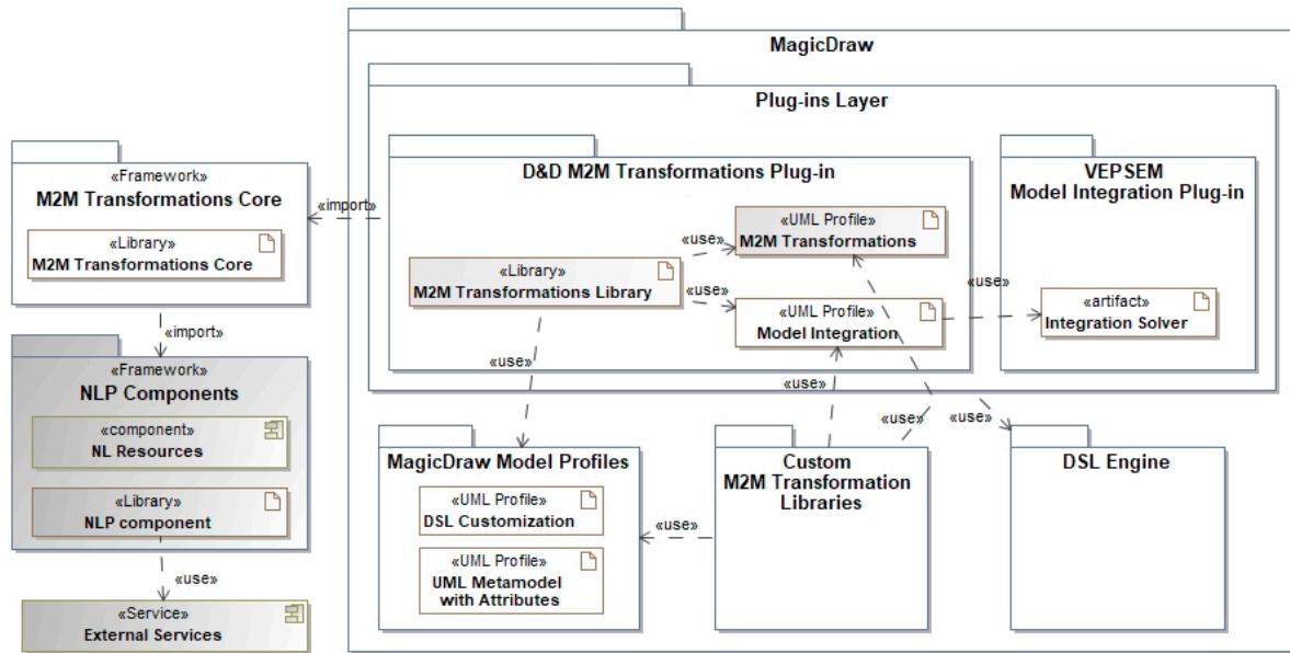
Figure 4. Implementation architecture of extended solution.
