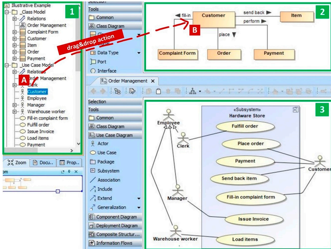
Figure 1. Illustrative example of partial model-to-model (M2M) transformation using drag-and-drop action.
