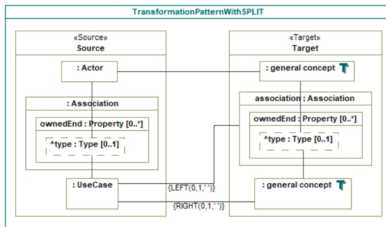
Figure 6. Sample transformation pattern with SPLIT.
