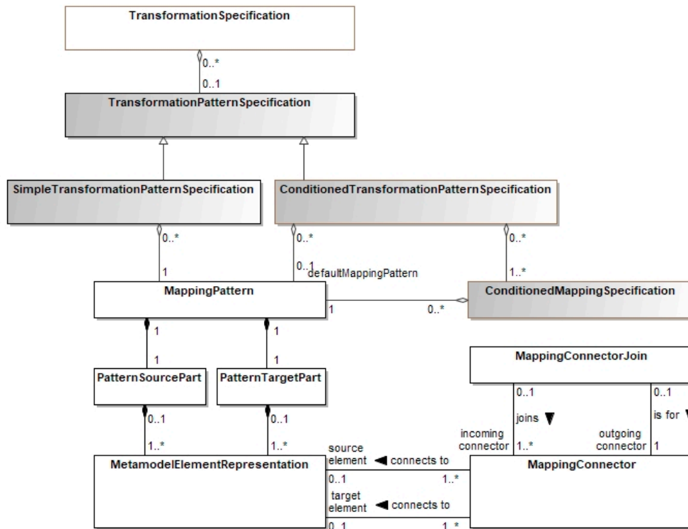
Figure 2. Extended metamodel of model-based M2M transformation.
