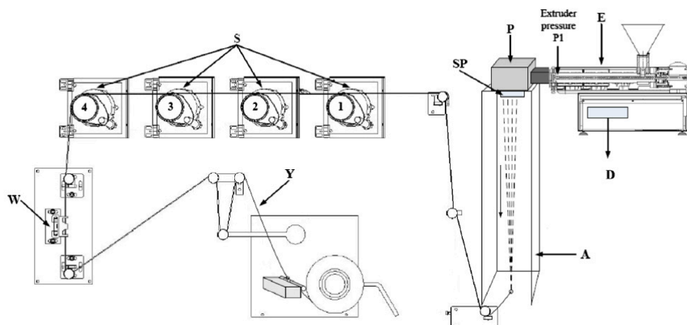
Figure 1. Principal scheme of the laboratory spinning equipment COLLIN ® CMF 100 (Dr. Collin GmbH, Maitenbeth, Germany): E—extruder; P—melting pump; SP—spinneret; A—air quench cabinet; D—display; S—stretching gadgets; W—whirling unit; Y—multifilament yarn from microfibers [26].
