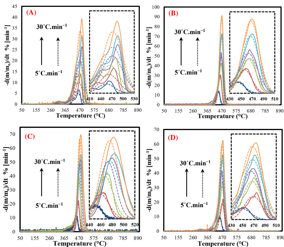
Figure 3. Experimental (solid lines) and calculated results (dotted lines) of the IPR model at heating rates 5–30 °C min -1 for (A) coffee, (B) chips, (C) chocolate, and (D) and mixed sample.
