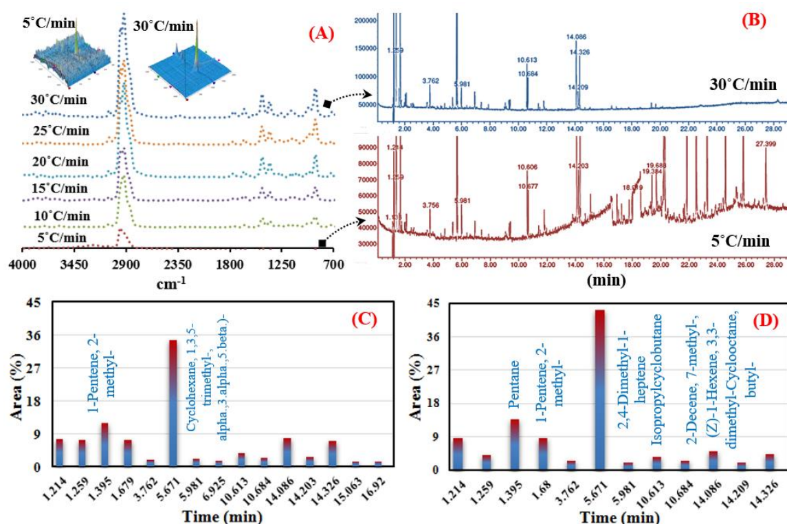
Figure 2. (A) 2D-3D FTIR analysis, (B) GC-MS analysis at 5 and 30\text{ }^{\circ}\text{C/min} , and (C,D) the obtained GC-MS compounds at 5 and 30\text{ }^{\circ}\text{C min}^{-1} .
