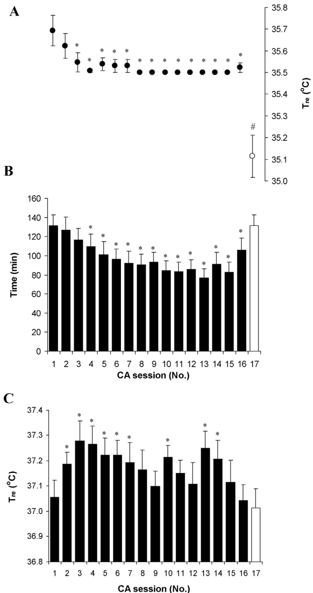
Figure 2. Cooling time and rectal temperature throughout the cold acclimation. Cooling time (B) and rectal temperature before (C) and after (A) cooling. * P < 0.05 , compared with CA-1; # P < 0.05 , compared with CA-17. Values are means \pm SEM. doi:10.1371/journal.pone.0094698.g002
