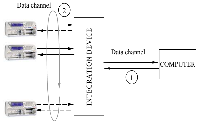
Fig. 3. Data streams
