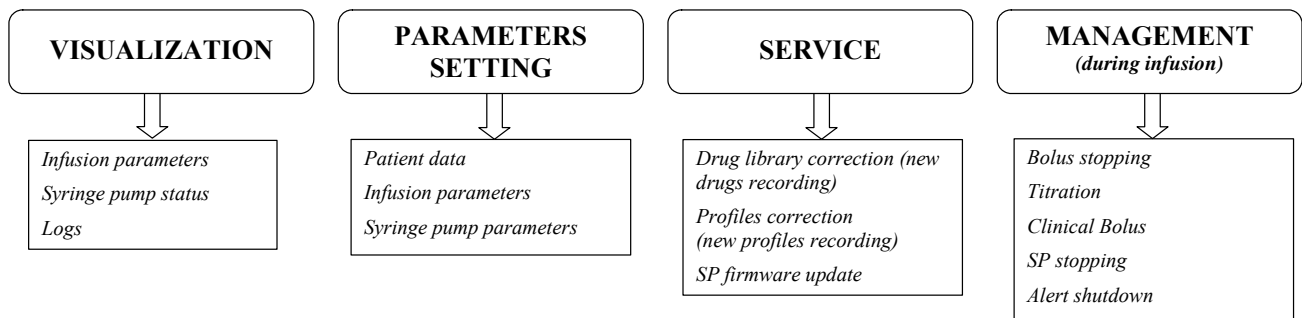
Fig 5. Command groups
