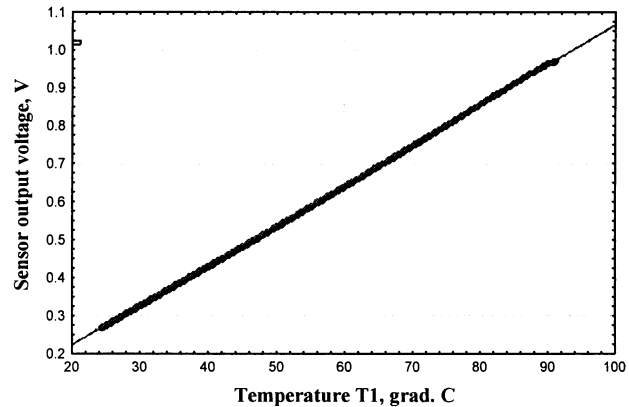
Fig. 4. The dependence of the sensor output voltage on the temperature
