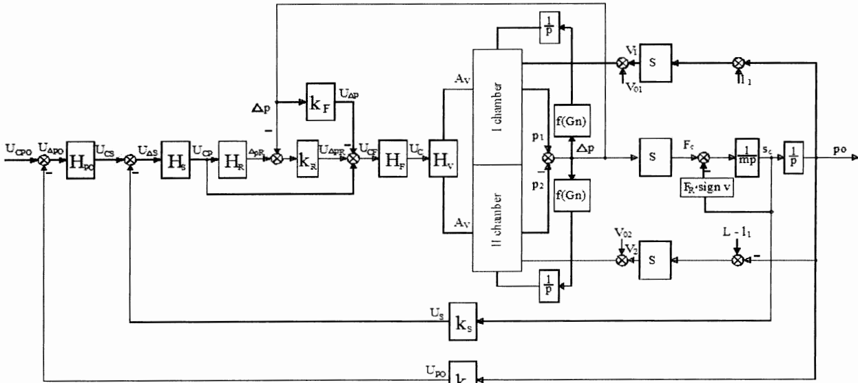
Fig. 1. The structural model of an electropneumatic position control system
