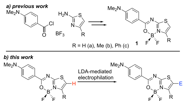
Figure 1. (a) Synthesis of thiazolo[3,2- c ][1,3,5,2]oxadiazaborinine dyes and (b) modification of thiazolo[3,2- c ][1,3,5,2]-oxadiazaborinines via LDA-mediated electrophilation reaction.
