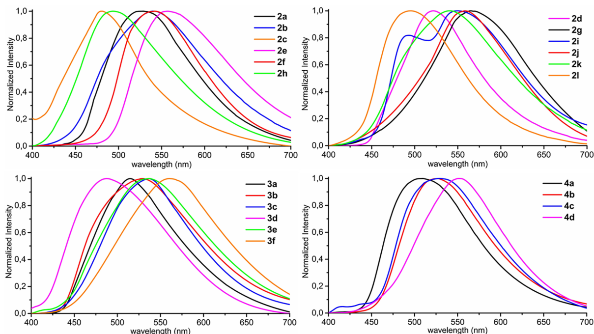
Figure 4. Normalized solid-state emission spectra of complexes 2a–l , 3a–f , and 4a–d ( \lambda_{\text{ex}} = 374 \text{ nm} ).
