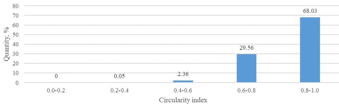
Figure 17. Distribution of pellets according to roundness.
