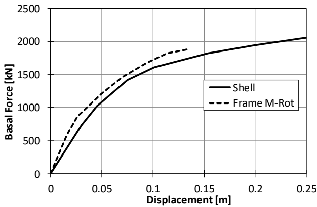
Fig. 10 Uniform loading in direction y
