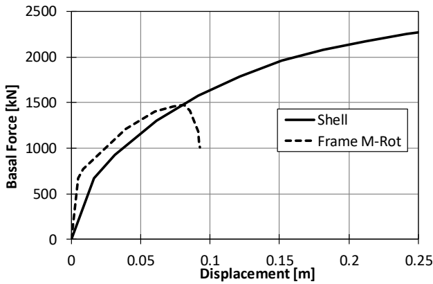
Fig. 9 Uniform loading in direction x
