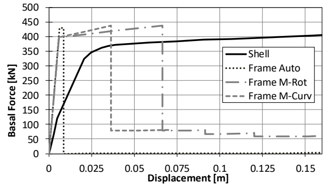
Fig. 7 Modal loading
