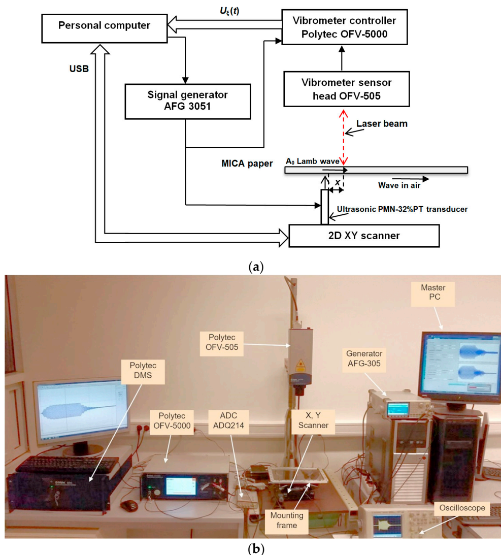
Figure 19. Experimental setup.
