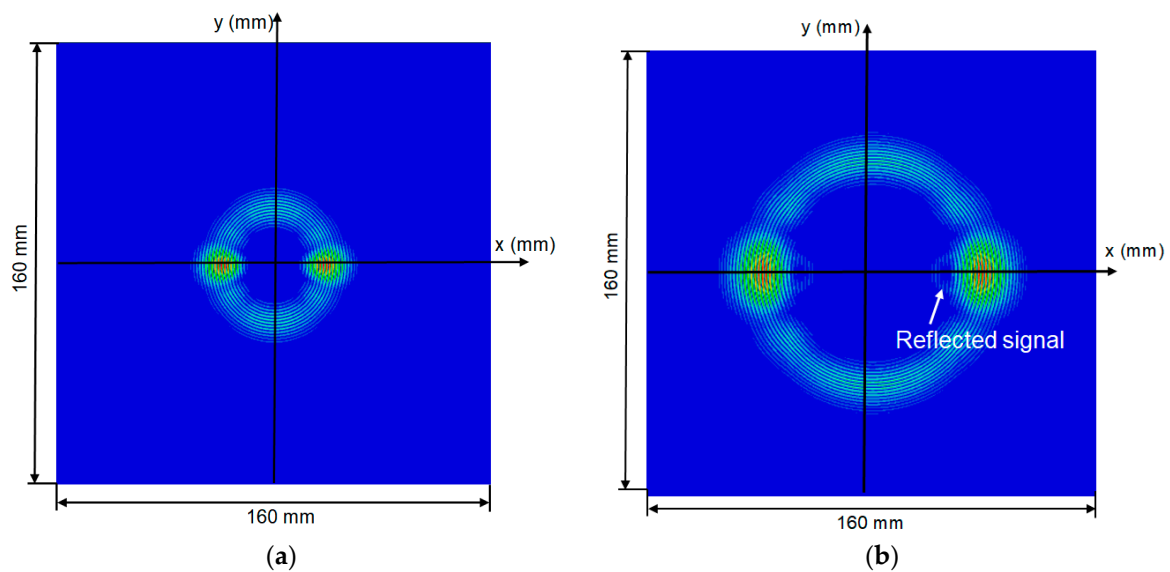
Figure 4. Spatial distributions of the normal particle velocity at two different time instants: (a) 150 \mu\text{s} ; (b) 246 \mu\text{s} .
