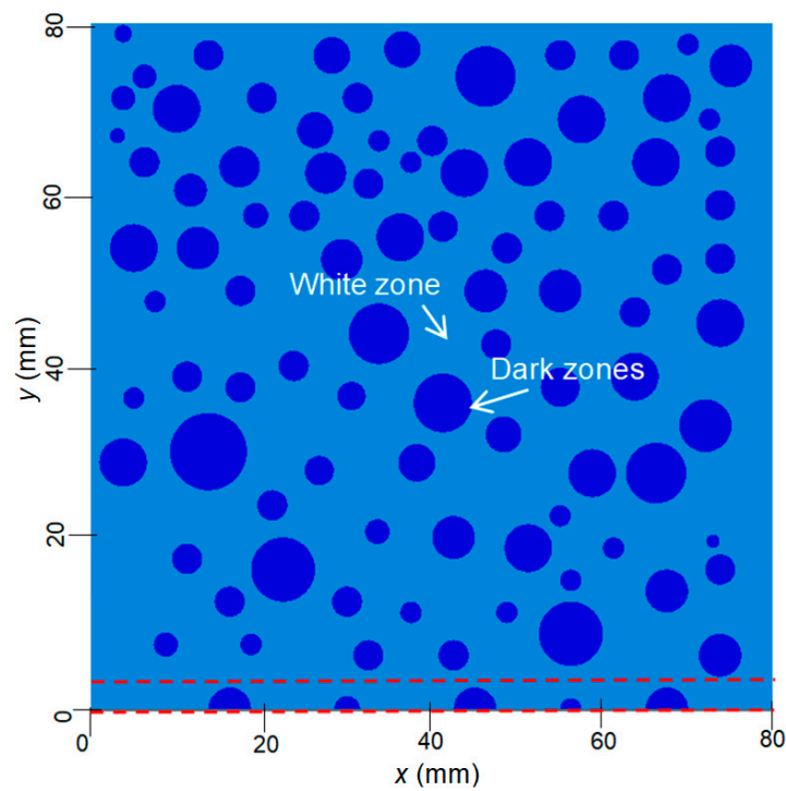
Figure 12. 2D spatial distribution of circular non-uniformities in mica paper with dimensions 80 \times 80 mm (red lines are y = 0 mm and y = 3 mm).
