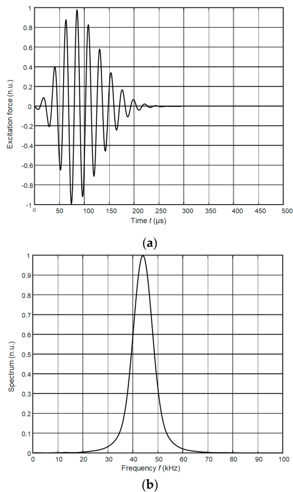
Figure 2. The waveform (a) and the spectrum of the excitation force (b); n.u. represents normalized units.
