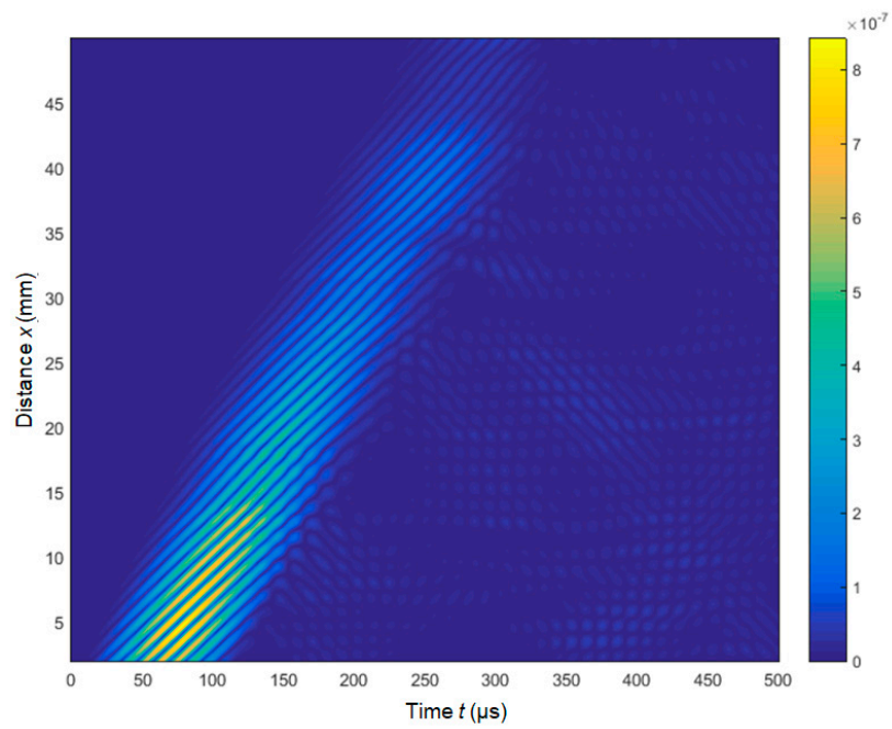
Figure 14. The simulated B-scan of the mica paper sample with multiple circular non-uniformities.
