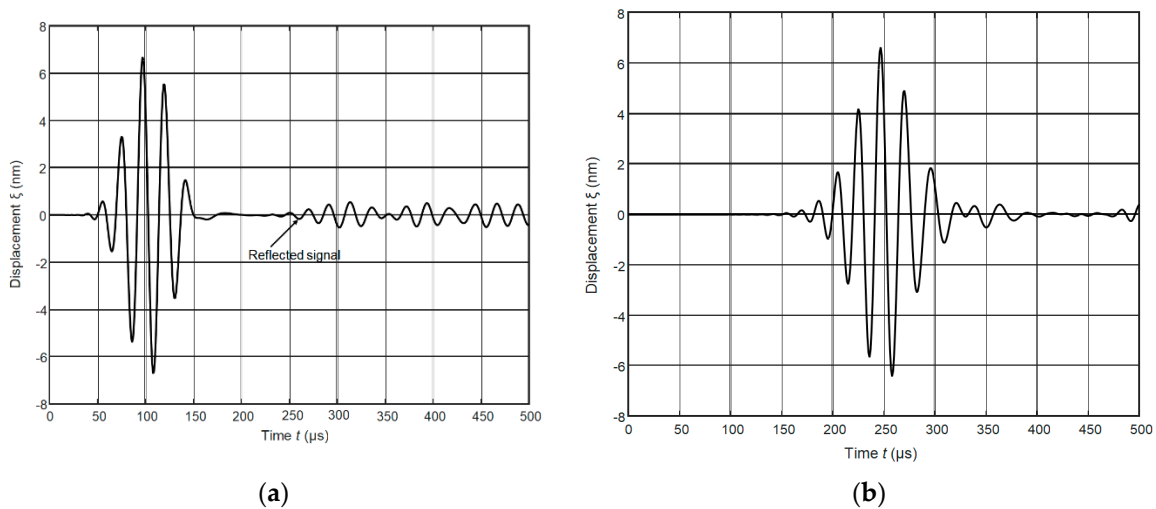
Figure 5. Ultrasonic pulses at two different distances from the 1 \times 5 \text{ mm}^2 excitation zone: (a) 10 mm; (b) 40 mm.
