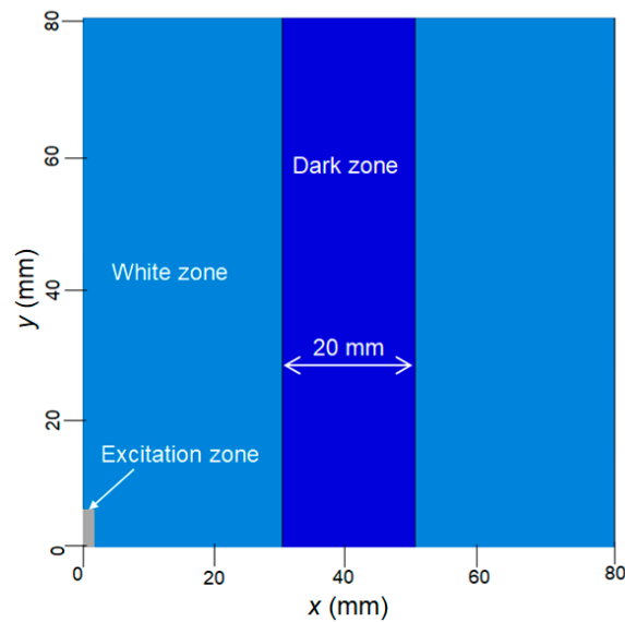
Figure 3. Sample of the mica paper with two zones with different elastic properties.
