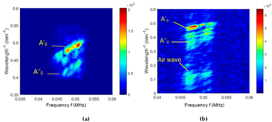
Figure 22. 2D spectra of the contact (a) and of the air-coupled B-scans (b).
