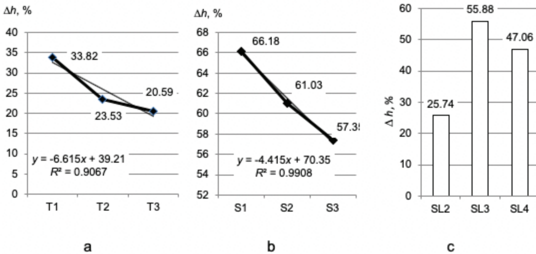
Figure 4. Percentage changes in the embroidery sample thickness \Delta h applying SL1 embroidery threads for both Tatami filling (T1, T2, and T3) (a) and Satin filling (S1, S2, and S3) (b) and for different embroidery threads SL2, SL3, and SL4 with S2 technological parameter set (c) (Note: Measurement error varied from 0.75% to 3.42%).
