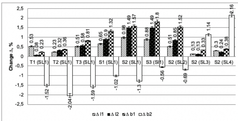
Figure 5. The changes in embroidery dimensions: widths ( \Delta b_1 and \Delta b_2 ) and lengths ( \Delta l_1 and \Delta l_2 ) in the case of applying SL1 embroidery threads for both Satin (S1, S2, and S3) (a) and Tatami filling (T1, T2, and T3) (b) and for different embroidery threads SL2, SL3, and SL4 with S2 set of technological parameters (c).
