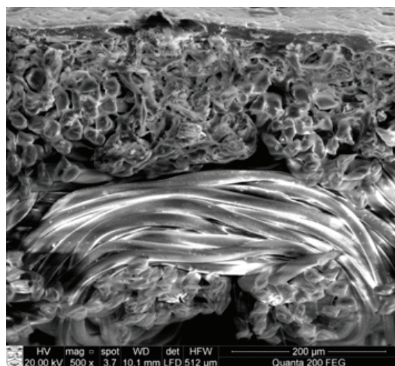
Figure 1. SEM images of the PU-coated PES knitted fabric's cross-sections: course (a) and wale (b).
