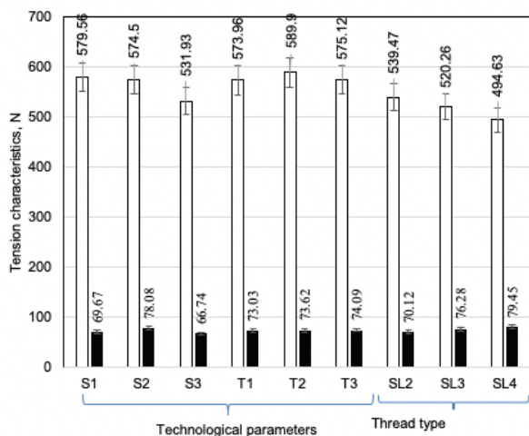
Figure 6. Force at break (white columns) and elongation at break (black columns) of embroidery applying SL1 embroidery threads for both Satin filling (S1, S2, and S3) and Tatami filling (T1, T2, and T3) as well as for different embroidery threads SL2, SL3, and SL4 with S2 technological parameters.
