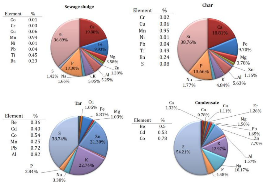
Fig. 3. Elemental distribution in sewage sludge, char, tar and condensate. The results in tables near the diagrams presented the values in range between 0.01 % and 1 %.
