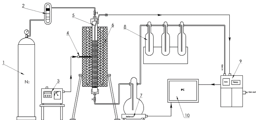
Fig. 2. The schematic configuration of pyrolysis experiment. 1. Nitrogen gas 2. Flowmeter 3. Temperature controller 4. Thermocouple of reactor 5. Thermocouple of sludge feed 6. Furnance 7. Balance 8. Ice bath 9. Gas analyzer 10. PC
