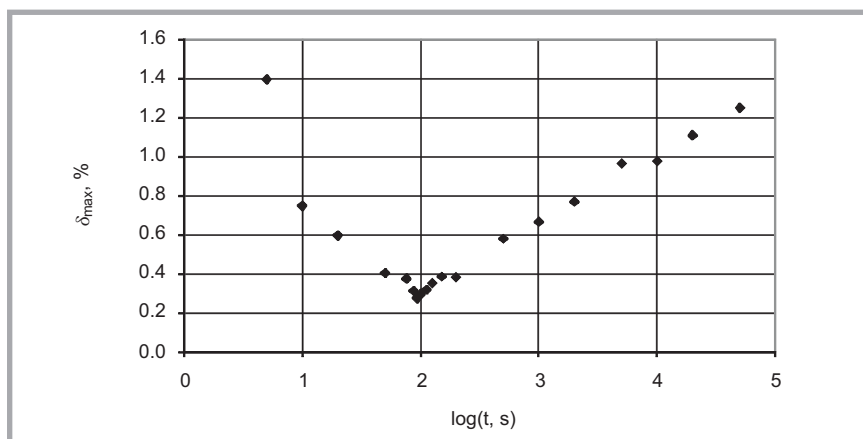
Figure 4. Dependence of maximum relative error between experimental and calculated values ( \delta_{\max} ) for break-point selected.
