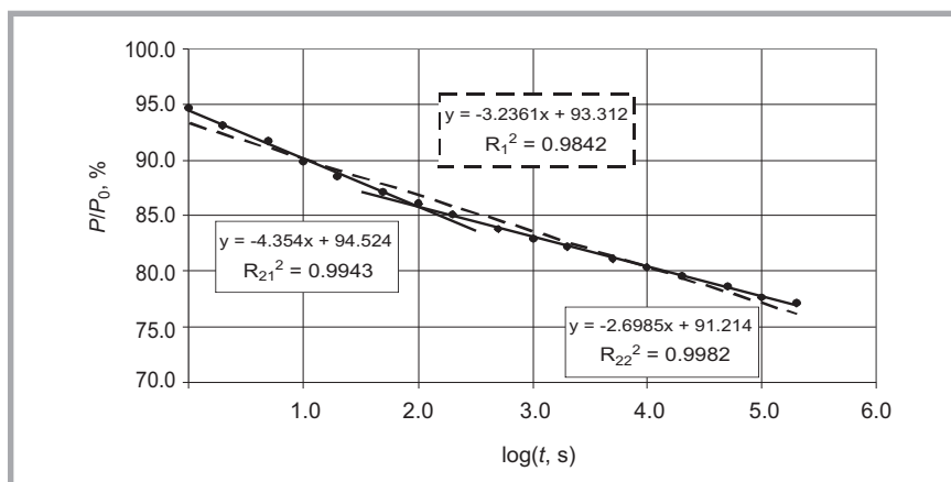
Figure 2. Description of relaxation process of polyester yarn: 1 – described by one straight line, 2 – described by two straight lines ( 2_1 – line of first part ( \log t = 0 - 2 ), 2_2 – line of second part ( \log t = 2 - 5.3 )).
