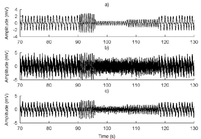
Fig. 5. Synthetic clean and noisy PPG signals: clean PPG signal (a), noisy PPG signal (SNR 0 dB) (b), noisy PPG signal (SNR 10 dB) (c).
