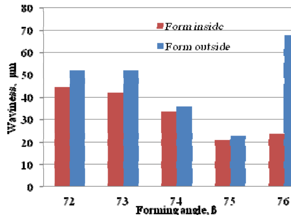
Fig. 11 Waviness of formed parts (AW1050)
