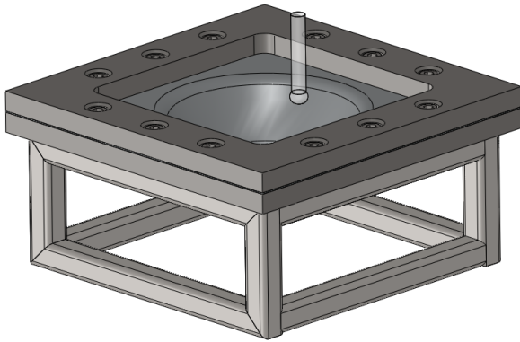
Fig. 1 SPIF technological equipment
