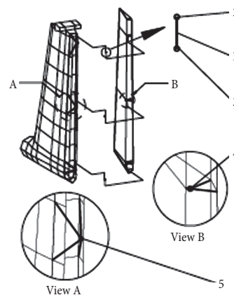
Fig. 2. Modelling of control surfaces hinges: 1 – beam element; 2, 3 – nodes of the beam element; 4, 5 – multipoint constraints
