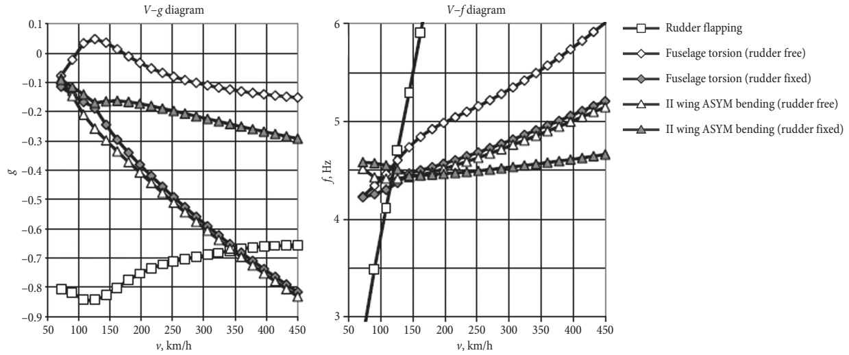
Fig. 8. V - g and V - f diagrams of sailplane LAK-17B with 18 m wing span
