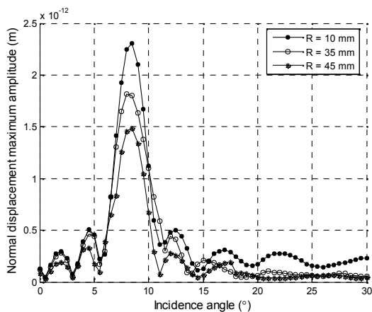
Fig. 6. Dependency of A_0 mode normal displacement amplitude maximum positive peak for 2 mm aluminium plate using 500 kHz excitation signal.
