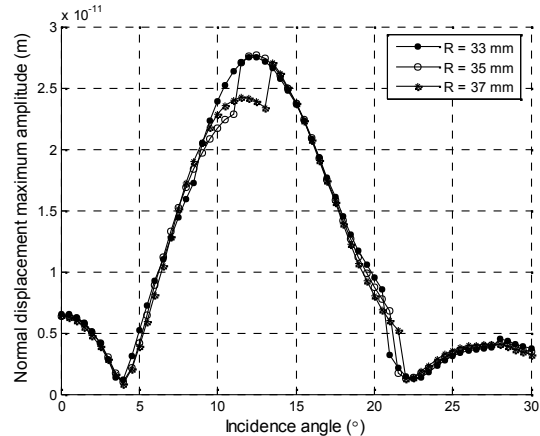
Fig. 8. Dependency of A_0 mode normal displacement amplitude maximum positive peak for 2 mm aluminium plate using 150 kHz excitation signal.
