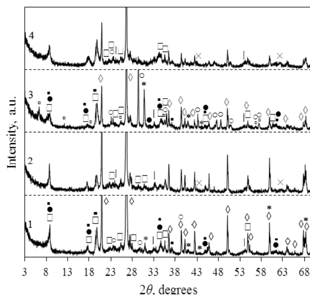
Fig. 5. X-ray diffraction pattern of calcined Dukstyna and Saltiskiai clays at different temperatures: 1 – D-600 °C; 2 – D-860 °C; 3 – Š-600 °C; 4 – Š-730 °C. Indexes: ● – illite; ■ – muscovite; ◆ – quartz; ○ – calcite; * – dolomite; | – hematite; ◻ – chlorite; – potassium aluminum silicate; × – periclase
