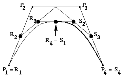
Figure 1. Illustration of the De Casteljau's algorithm
