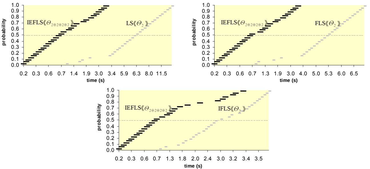
Figure 14. Time-to-target plots for the TSPLIB instance gr96
