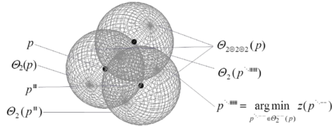
Figure 5. Graphical representation of the neighborhood \Theta_{2\oplus 2\oplus 2}
