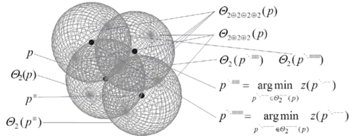
Figure 6. Graphical representation of the neighborhood \Theta_{2\oplus 2\oplus 2\oplus 2}
