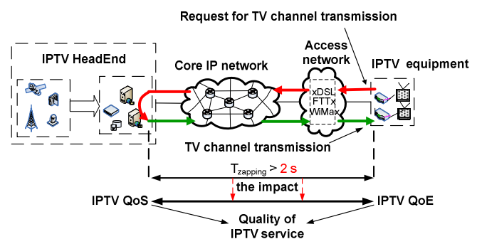
Fig. 1. The influence of the channel change process to the quality of IPTV service.
