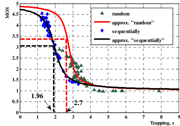
Fig. 5. The relationship between the user perceived quality of service (MOS) and TV channels zapping times using the different methods for IPTV channel search.
