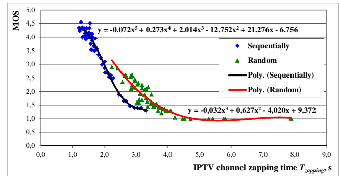
Fig. 4. The dependency of MOS values and IPTV channel zapping times and it polynomial approximation.
