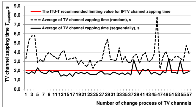
Fig. 2. IPTV channel zapping time using the different methods for TV channel search and selection [9].
