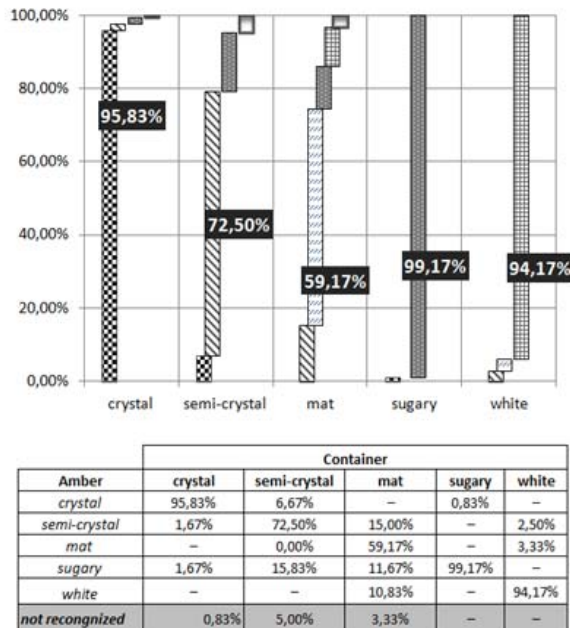
Fig. 10. Ambers classification results according to tree classifier
