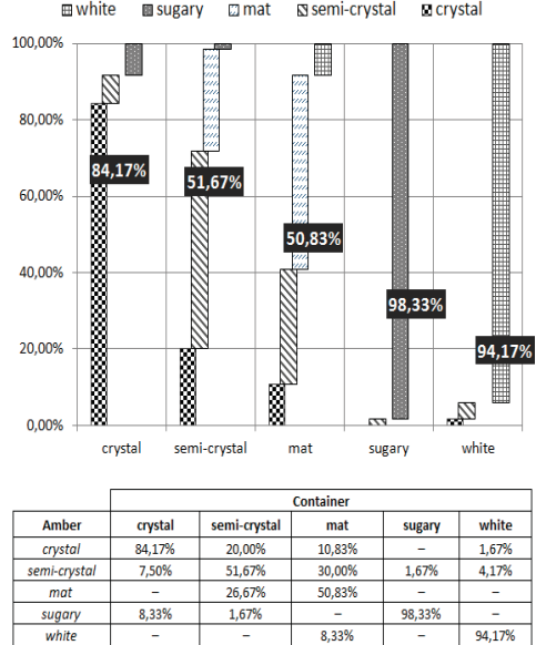
Fig. 6. Ambers classification results according to HSV color features
