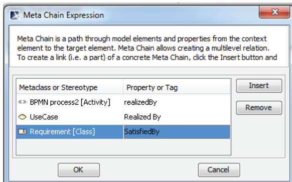
Figure 6. A metachain expression for search of indirectly related components
