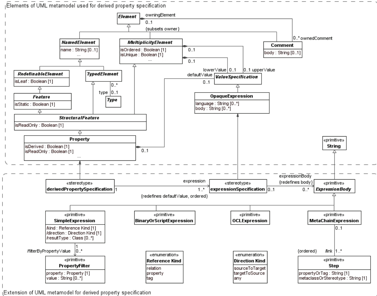
Figure 3. UML metamodel extended with derivedPropertySpecification stereotype for specifying derived properties
