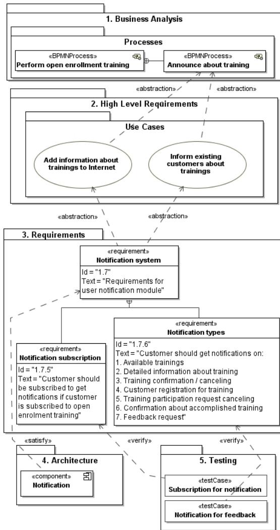
Figure 2. Training Organization System model (fragment)
