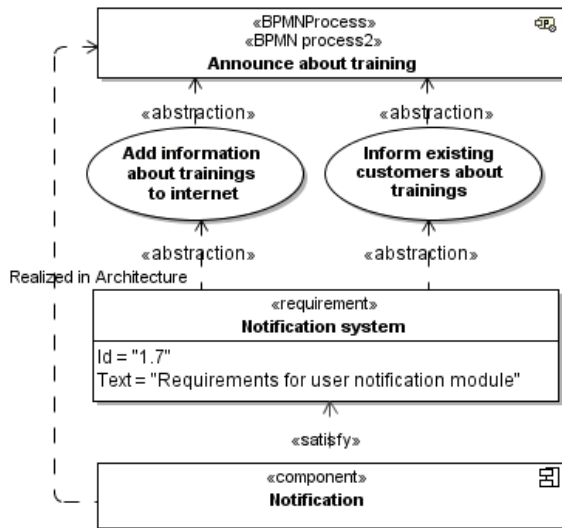
Figure 5. A derived property “Realized in Architecture”
