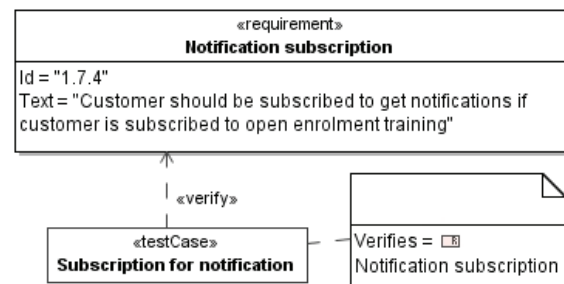
Figure 4. A derived property “Verifies” is calculated on the base of abstraction “verify”
