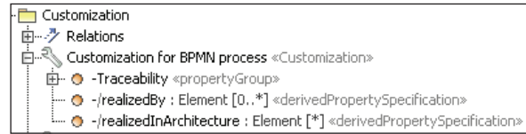
Figure 8. Specification of derived properties of a customization class in MagicDraw CASE tool
