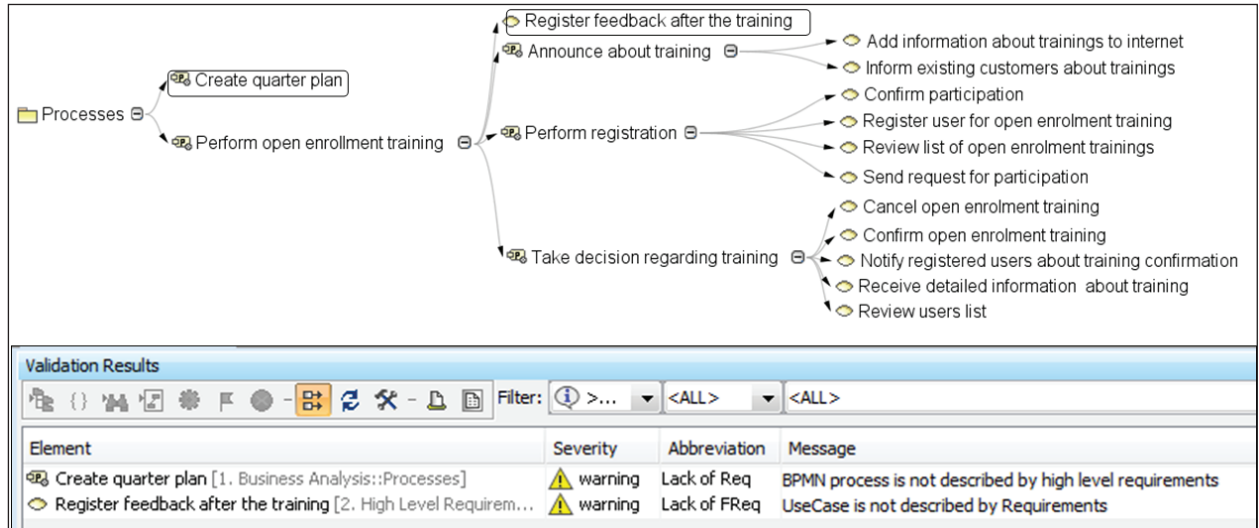
Figure 12. Validation results below Relation Map inform about uncovered project parts, e.g. business process and high level re-quirements
