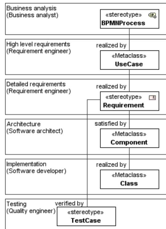
Figure 1. The structure of the Training Organization System project
