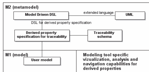
Figure 7. Derived Property Based Traceability Framework
