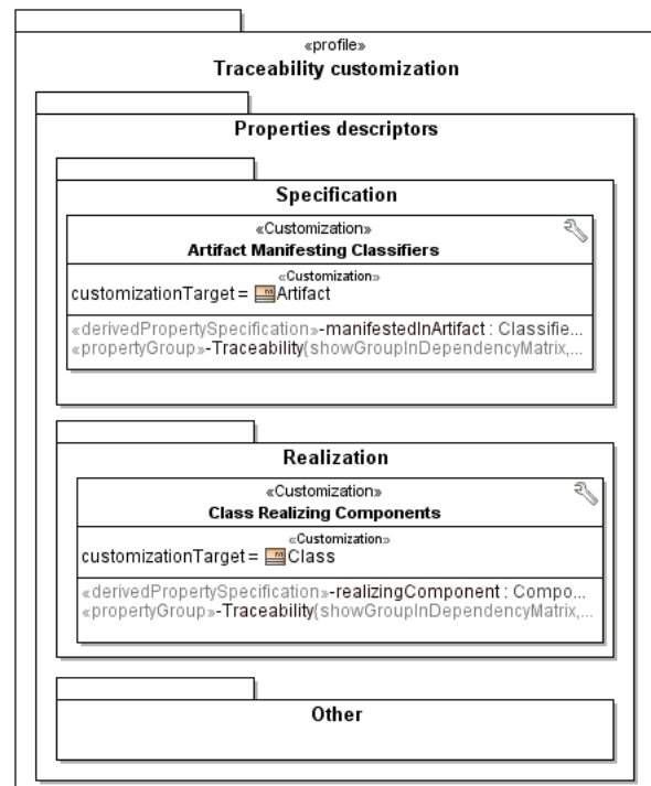
Figure 9. The traceability schema “Traceability customization” as a module
