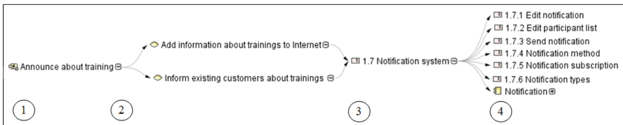
Figure 10. Relation Map – graph based visualization enabling analysis of multilevel relations, e.g. from business analysis stage (1) to high level requirements (2), concrete requirements (3), and architecture (4)
