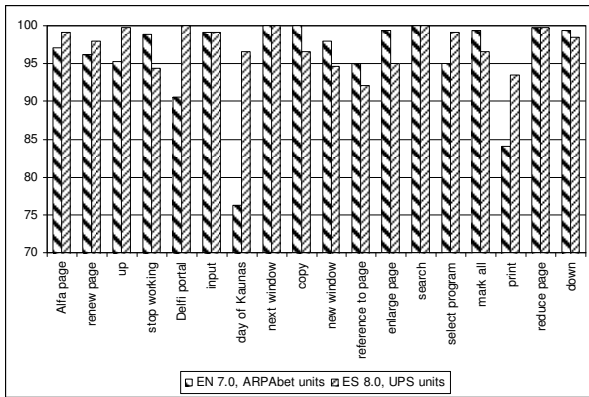
Fig. 2. The recognition accuracy of internet browsing Lithuanian commands using English and Spanish speech engines and different sets of transcriptions.
