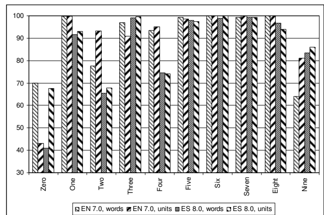
Fig. 1. The recognition accuracy of 10 Lithuanian voice commands using English and Spanish speech engines.
