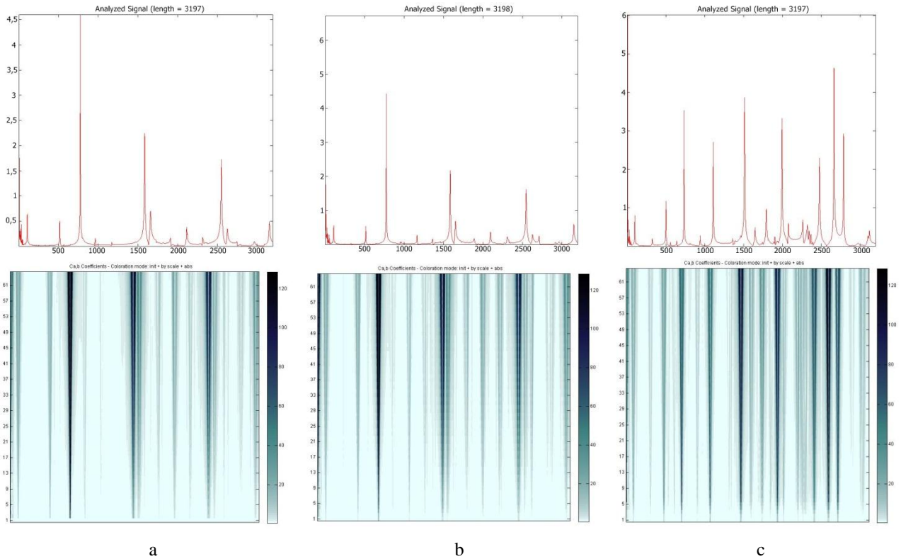
Fig. 9 The results of using Haar wavelet for defect detection with experimental data: a) floor without defect; b) floor with defect 1; c) floor with defect 3
