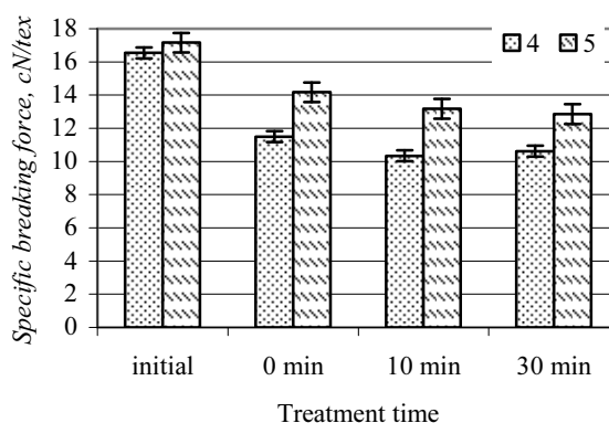
Fig. 9. The influence of treatment on cotton yarns specific breaking force: 4 – 4 th yarn, 5 – 5 th yarn
