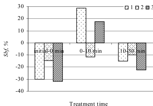
Fig. 8. The influence of treatment on PES yarns (marked as in Fig. 7) specific breaking force change
