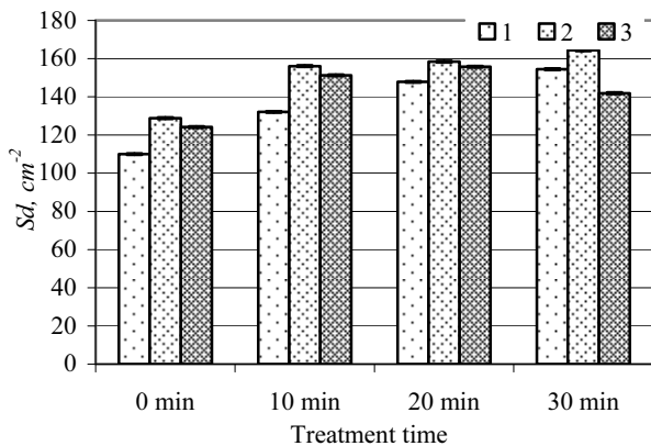
Fig. 1. The influence of stabilisation time on stitches density of PES/EL/PA knits: 1 – 1 st knit, 2 – 2 nd knit, 3 – 3 rd knit
