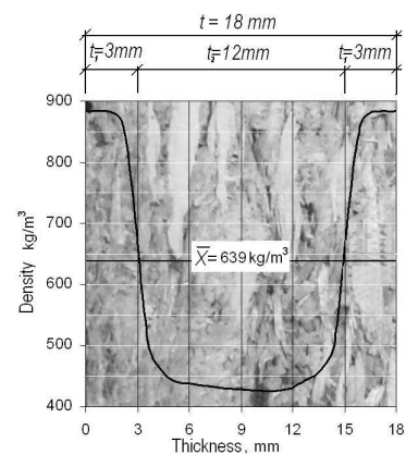
Fig. 4. Density distribution of particleboard in the thickness direction: thickness of particleboard t = 18 mm, thickness of outer layers t_1 = 3 mm; thickness of inner layer t_2 = 12 mm
