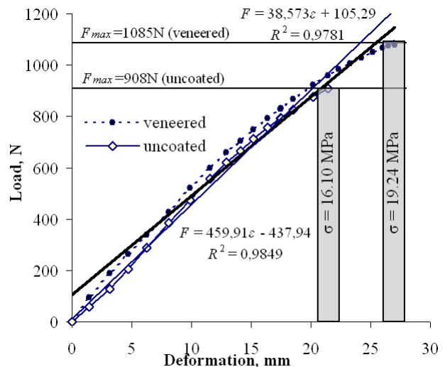
Fig. 10. Effect of veneering on bending strength of miter corner joint
