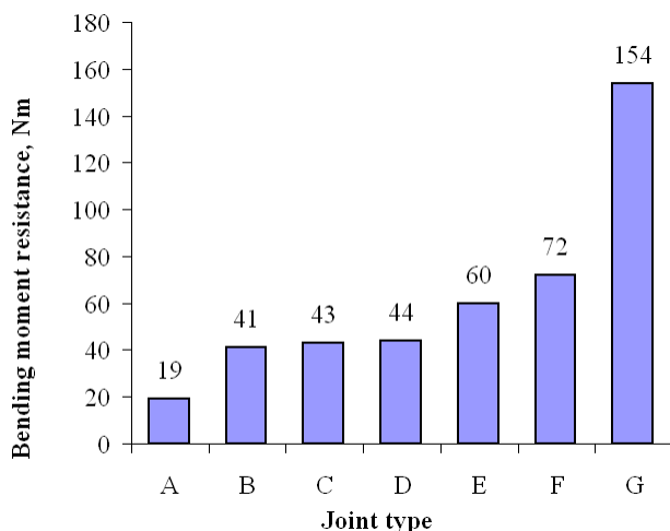
Fig. 12. Joint strength dependence on joint type: A – cam connecting fittings [14]; B – TZ connecting fittings [15]; C – bisquit joint [16, 17]; D – tongue and groove joint [18]; E – screw joint [19–21]; F – multidowel joint [22]; G – mitre joint
