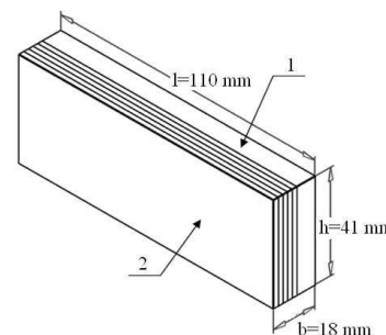
Fig. 1. Slicing scheme for density distribution of particleboard in the thickness direction: l , h , b – length 110 mm, height 41 mm and thickness 18 mm of specimen in mm; 1 – particleboard; 2 – 9 cut off layers
