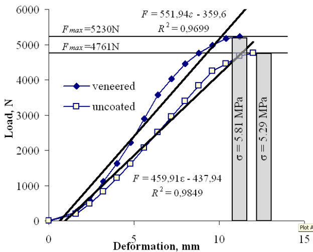
Fig. 7. Effect of veneering on tensile strength of specimen
