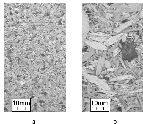
Fig. 5. Optical views of wood particle in the outer (a) and inner (b) layers of the particleboard
