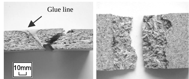
Fig. 8. View of uncoated specimen after tensile tests (edge and face views)
