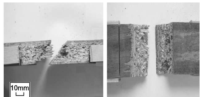
Fig. 9. View of veneered specimen after tensile tests (edge and face views)
