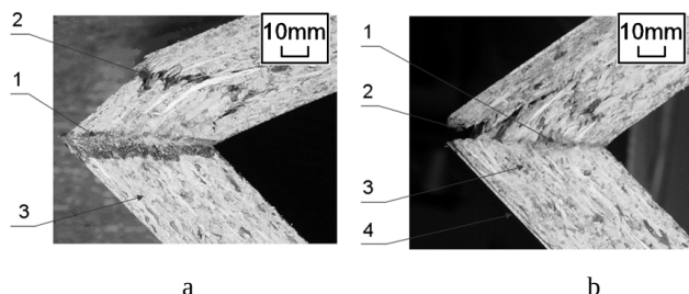
Fig. 11. Failure scheme of uncoated (a) and veneered (b) mitre joint: 1 – glue line; 2 – fracture crack; 3 – particleboard; 4 – wood veneer
