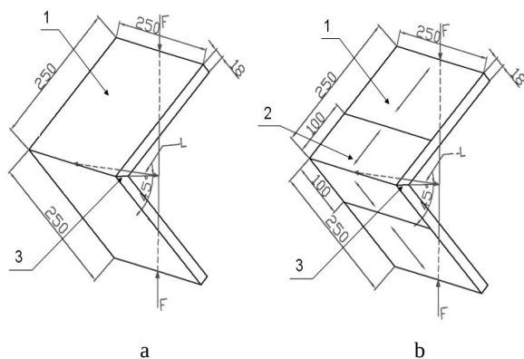
Fig. 3. Specimen scheme of uncoated (a) and veneered (b) mitre joints: 1 – panel (particleboard); 2 – wood veneer; 3 – glue line (PVA); F – load direction
