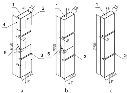
Fig. 2. Tensile specimen and loading scheme: a – veneered specimen (miter bond), b – uncoated specimen (miter bond), c – uncoated specimen (solid): 1 – particleboard, 2 – wood veneer, 3 – cuts (half of specimen thickness), 4 – plywood, 5 – PVA glue line, F – load direction
