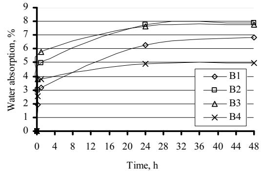
Fig. 2. Water absorption kinetics of concrete
