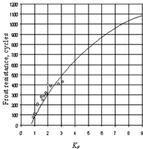
Fig. 1. The dependence of frost resistance of concrete on the predicted criterion of concrete of freezing and thawing resistance [1]
