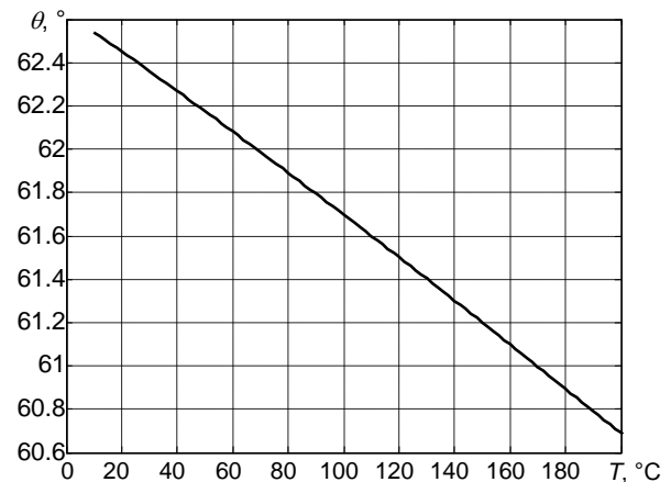
Fig. 3. Angle of the deflection of the waveguide at different temperatures.
