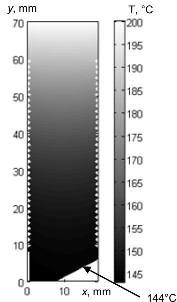
Fig. 2. Temperature distribution in the titanium waveguide.
