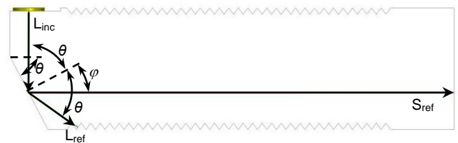
Fig. 1. Schematic diagram of the waveguide with mode conversion.
