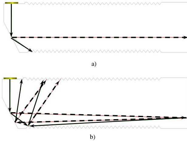
Fig. 4. Ultrasonic waves propagation paths in a titanium waveguide. a – 20°C; b 144°C. Solid line - longitudinal wave, dashed line - shear wave.
