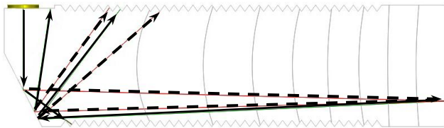
Fig. 6. Ultrasonic waves propagation paths in a waveguide with temperature gradient. Solid line - longitudinal wave, dashed line - shear wave.
