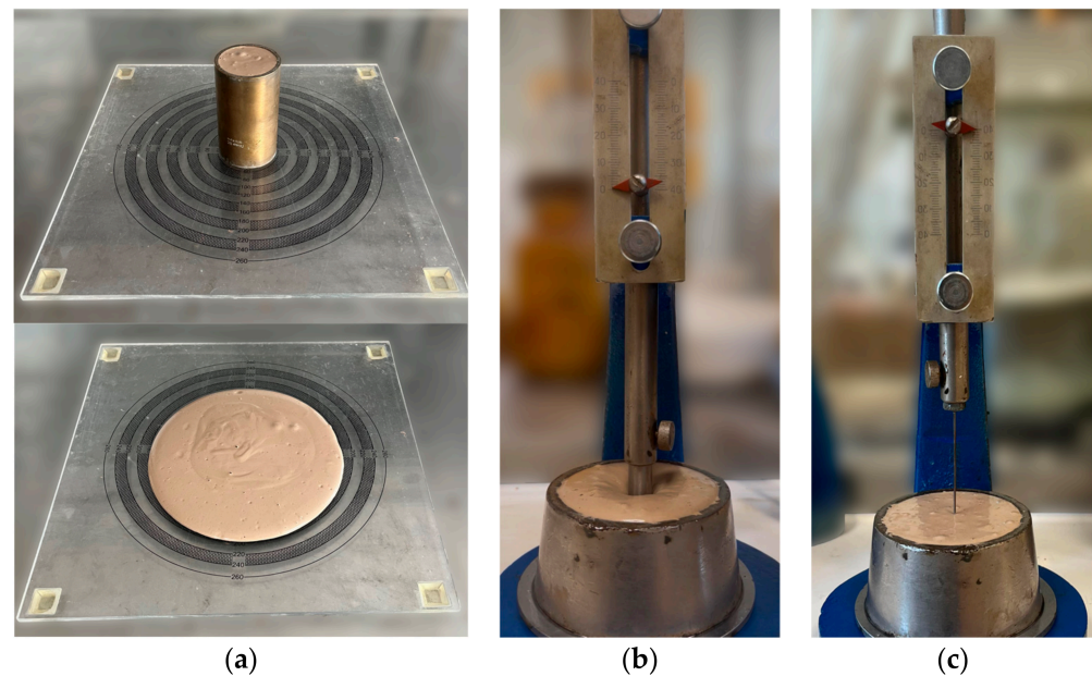
Figure 5. Fresh-state geopolymer properties: (a)—flowability (Suttard viscometer); (b)—consistency (Vicat plunger); (c)—setting time (Vicat needle).
