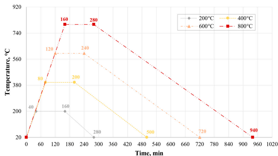
Figure 4. Applied temperature schedules for binder testing at target exposures of 200, 400, 600 and 800 °C.
