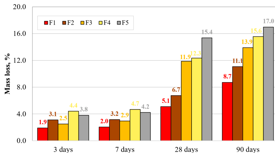
Figure 10. Change in mass throughout drying shrinkage.
