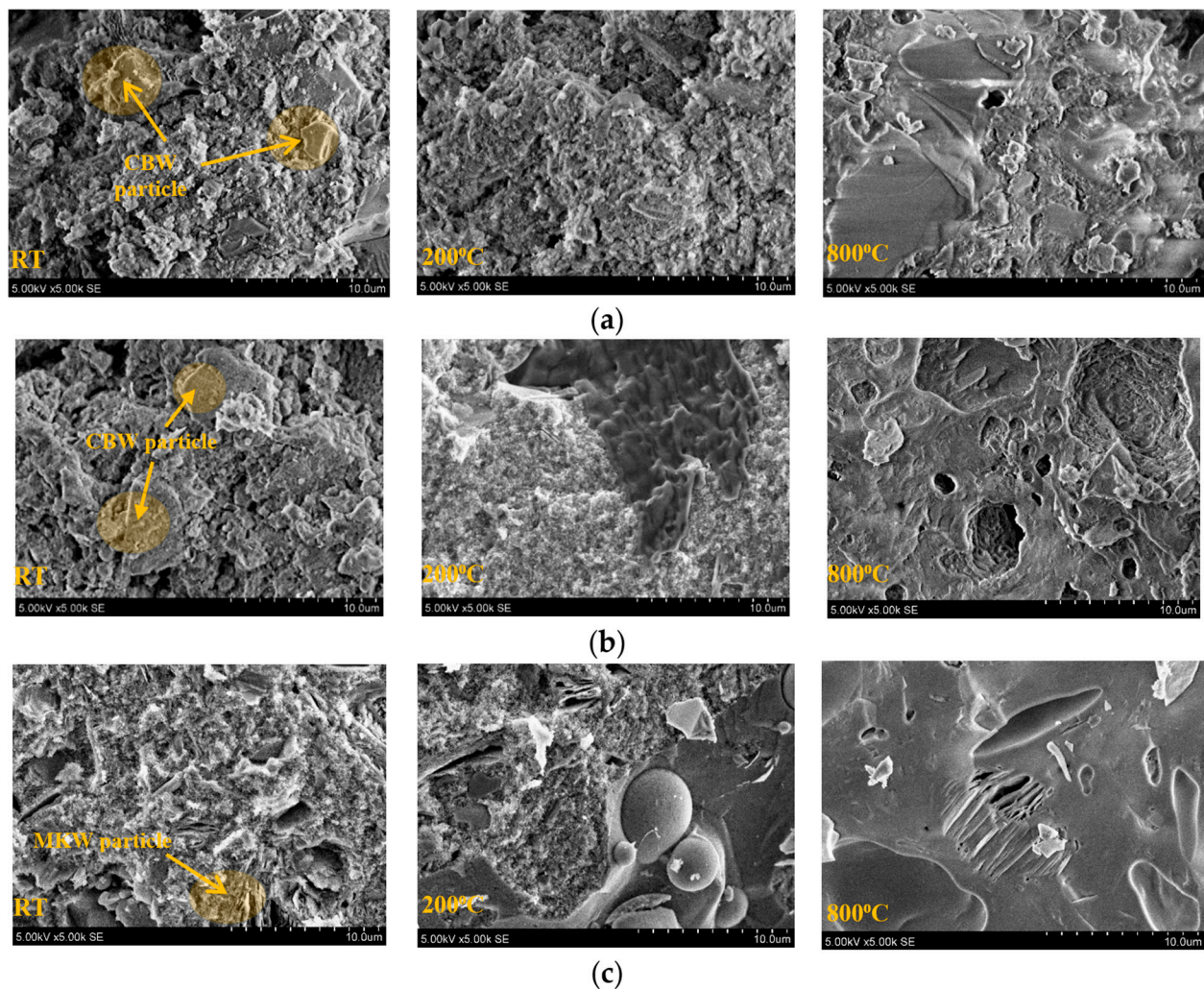
Figure 18. SEM images of geopolymer binder at room temperature, 200 °C, and 800 °C for compositions (a)—F1, (b)—F3, and (c)—F5.
