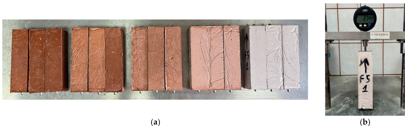
Figure 8. Geopolymer drying shrinkage test: (a)—binder prism specimens (F1–F5); (b)—length change measurement.
