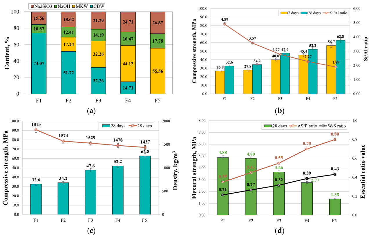
Figure 7. Mechanical properties of geopolymer binder: (a)—composition proportions; (b)—relationship between compressive strength at 7 and 28 days and Si/Al ratio; (c)—relationship between compressive strength and density at 28 days; (d)—relationship between flexural strength, AS/P and W/S ratio.
