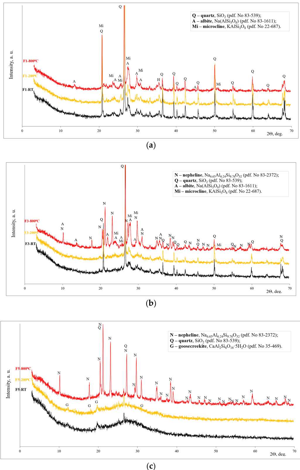
Figure 16. Mineralogical changes in geopolymer binders revealed by XRD analysis at room temperature, 200 °C, and 800 °C for compositions: (a)—F1, (b)—F3, (c)—F5.
