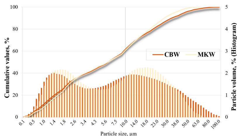
Figure 2. Precursor materials particle size distribution.
