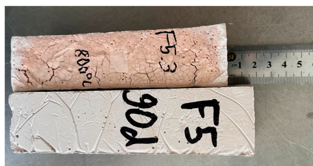
Figure 13. Visualization of extreme thermal shrinkage at 800 °C in composition F5.
