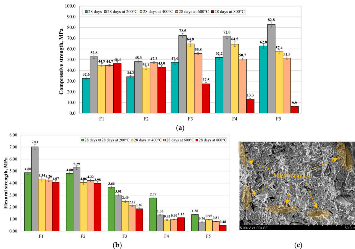
Figure 14. Mechanical properties of geopolymer binder after elevated temperature exposure: (a)—compressive strength; (b)—flexural strength, (c)—microcracks in composition F5 at 400 °C.
