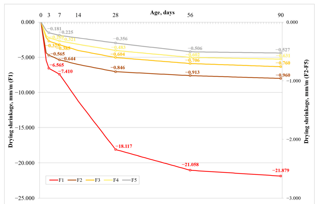
Figure 9. Geopolymer binder free-drying shrinkage after 90 days.
