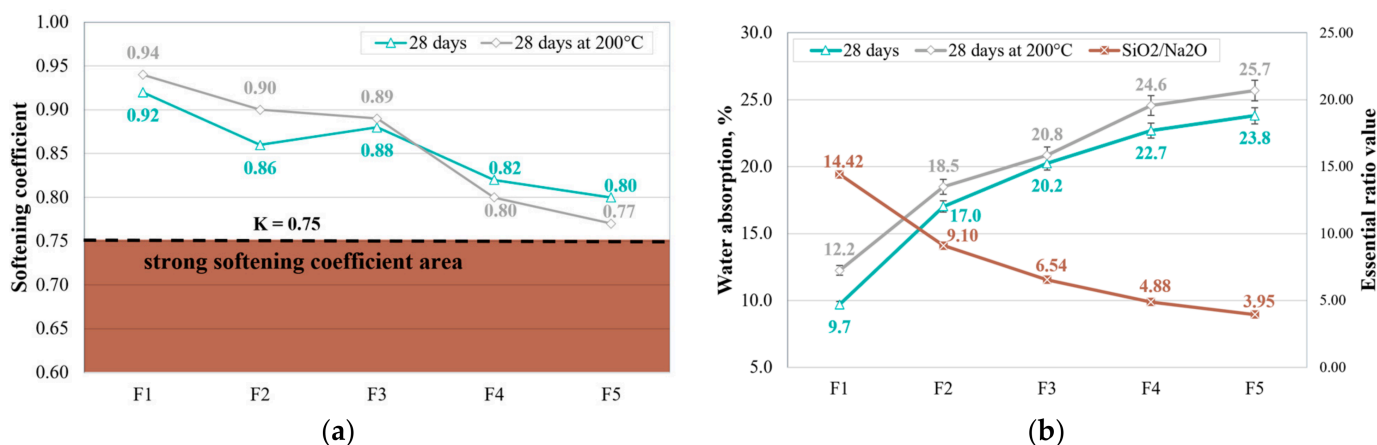
Figure 15. Water resistance of geopolymers after 28 days of curing and after thermal treatment at 200 °C: (a) softening coefficient; (b) water absorption.
