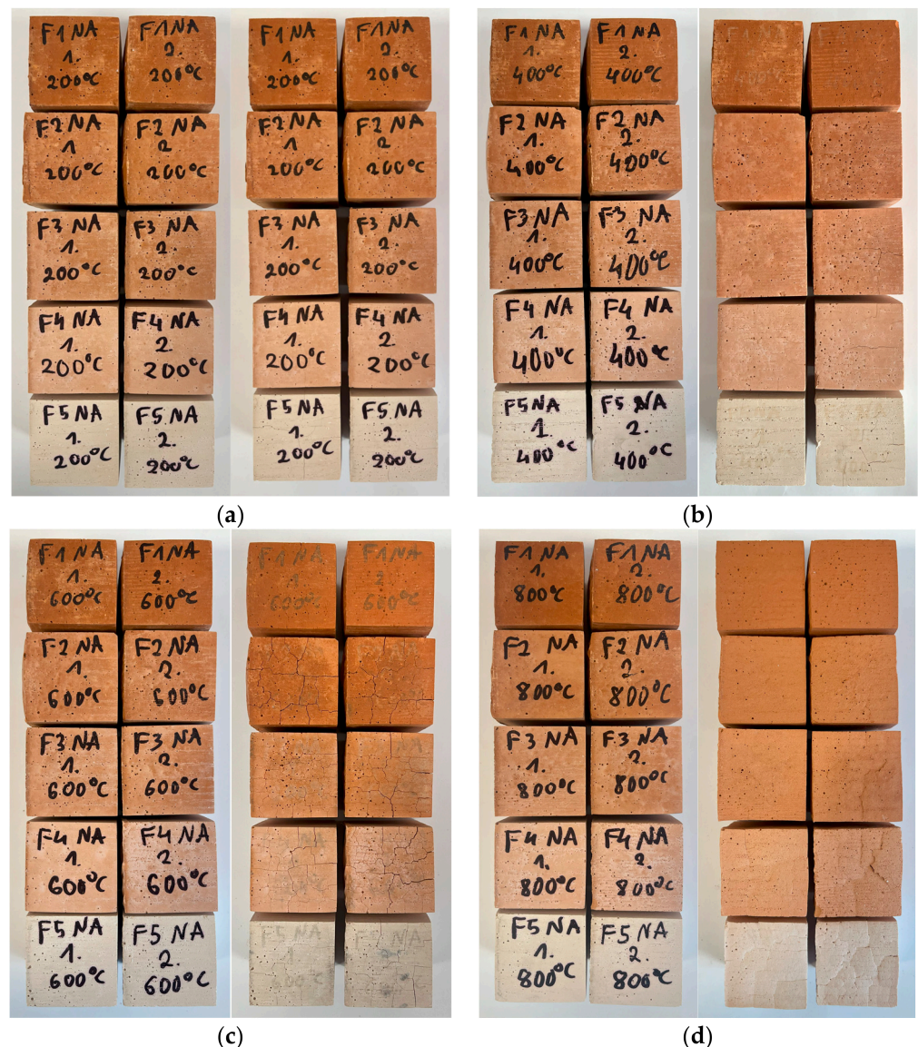
Figure 11. Macroscopic images of geopolymer binder specimens before and after elevated temperature exposure: (a)—200 °C; (b)—400 °C; (c)—600 °C; (d)—800 °C.
