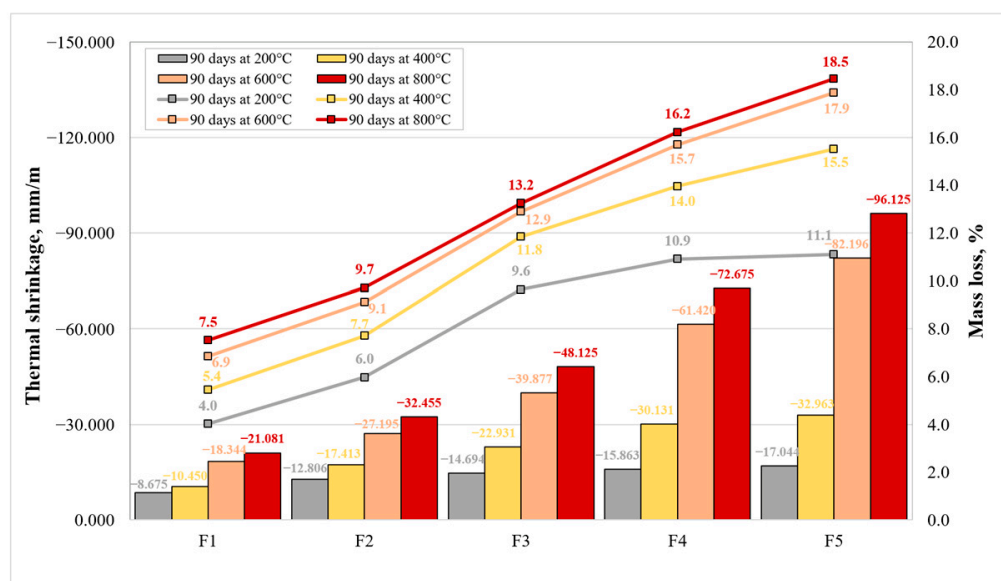
Figure 12. Relationship between thermal shrinkage and mass loss of the geopolymer binder after 90 days.
