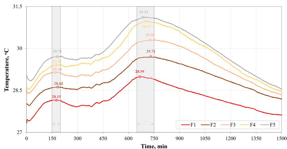
Figure 6. Heat evolution behavior of geopolymer pastes during hydration, as implied by temperature alterations over time.
