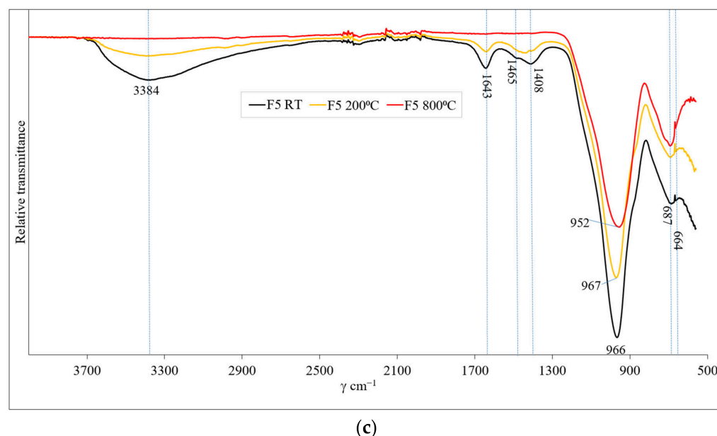
Figure 17. Mineralogical changes in geopolymer binders revealed by FT-IR analysis at room temperature, 200 °C, and 800 °C for compositions (a)—F1, (b)—F3, and (c)—F5.
