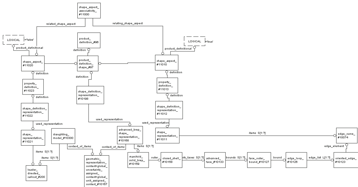
Figure 3. Example of associativity between a portion of the geometry (edge_curve) and the annotation (draughting_callout) using the old approach
