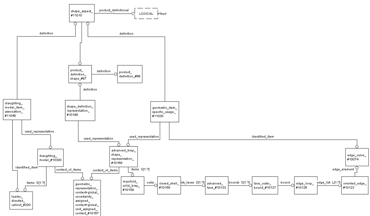
Figure 4. Example of associativity between the portion of the geometry (edge_curve) and the annotation (draughting_callout) using the new approach
