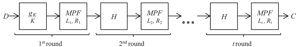
Figure 1. Encryption of t rounds matrix power cipher
