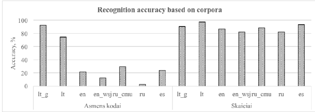
Fig. 2. Recognition results of single recognizers with every corpus.
