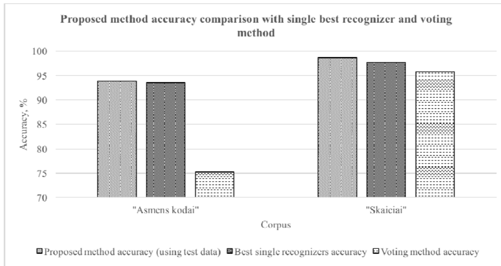
Fig. 4. Proposed method comparison with alternative methods.
