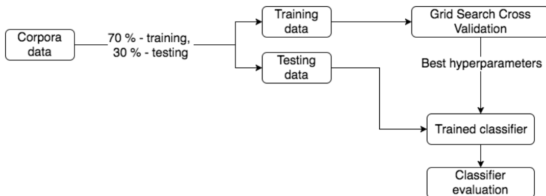
Fig. 3. Classifiers evaluation and hyperparameter tuning process.
