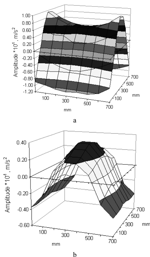
Fig. 2. Modes of wood particle boards finished with veneer on both sides: a – f = 89.7 Hz; b – f = 116.7 Hz
