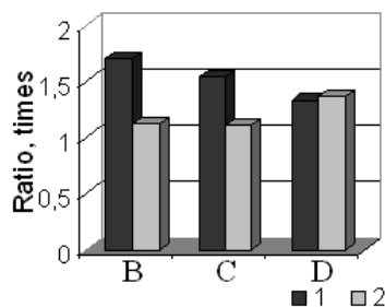
Fig. 5. The comparison of viscous-elastic properties of finished wood particle boards in two perpendicular bending directions: B – boards finished with veneer on both sides; C – boards finished with veneer on the one side and with compensatory paper on the other side; D – boards finished with melamine impregnated paper on both sides; here 1 – modulus of elasticity; 2 – coefficient of damping
