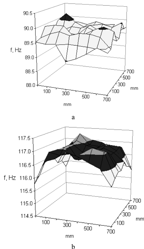
Fig. 3. Resonant frequency distribution low in the plane of the board with veneer finishing on both sides: a – when dealing with the first resonant frequency, b – when dealing with the second one
