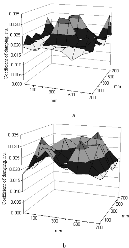
Fig. 4. Coefficient of damping distribution in the plane of the board with veneer finishing on both sides in the presence of: a – the first resonant frequency, b – the second resonant frequency
