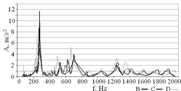
Fig. 1. Amplitude-frequency characteristics of boards: B – finished with veneer on both sides; C – finished with veneer on the one side and with compensatory paper on the other side; D – finished with melamine impregnated paper on both sides
