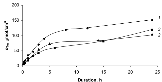
Fig. 3. Changes of tellurium concentration in the PA films chalcogenized in the 0.05 mol/dm 3 solutions of telluropentathionic compounds with time at 20 °C. PA chalcogenization precursor: 1 – K 2 TeS 4 O 6 ; 2 – H 2 TeS 4 O 6 ; 3 – Na 2 TeS 4 O 6
