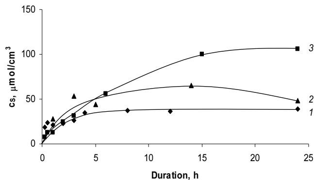
Fig. 1. Changes of sulfur concentration in the PA films chalcogenized in the 0.05 mol/dm 3 solutions of telluropentathionic compounds with time at 20 °C. PA chalcogenization precursor: 1 – K 2 TeS 4 O 6 ; 2 – H 2 TeS 4 O 6 ; 3 – Na 2 TeS 4 O 6
