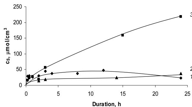
Fig. 2. Changes of sulfur concentration in the PA films chalcogenized in the 0.1 mol/dm 3 solutions of telluropentathionic compounds with time at 20 °C. PA chalcogenization precursor: 1 – K 2 TeS 4 O 6 ; 2 – H 2 TeS 4 O 6 ; 3 – Na 2 TeS 4 O 6
