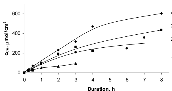
Fig. 5. Changes of copper concentration in the PA films chalcogenized in the solutions of sodium and potassium telluropentathionates with time at 20 °C. PA chalcogenization precursor (its concentration): 1 – Na 2 TeS 4 O 6 (0.1 mol/dm 3 ); 2 – Na 2 TeS 4 O 6 (0.05 mol/dm 3 ); 3 – K 2 TeS 4 O 6 ; (0.05 mol/dm 3 ); 4 – K 2 TeS 4 O 6 (0.1 mol/dm 3 )
