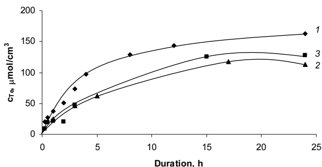
Fig. 4. Changes of tellurium concentration in the PA films chalcogenized in the 0.1 mol/dm 3 solutions of telluropentathionic compounds with time at 20 °C. PA chalcogenization precursor: 1 – K 2 TeS 4 O 6 ; 2 – H 2 TeS 4 O 6 ; 3 – Na 2 TeS 4 O 6
