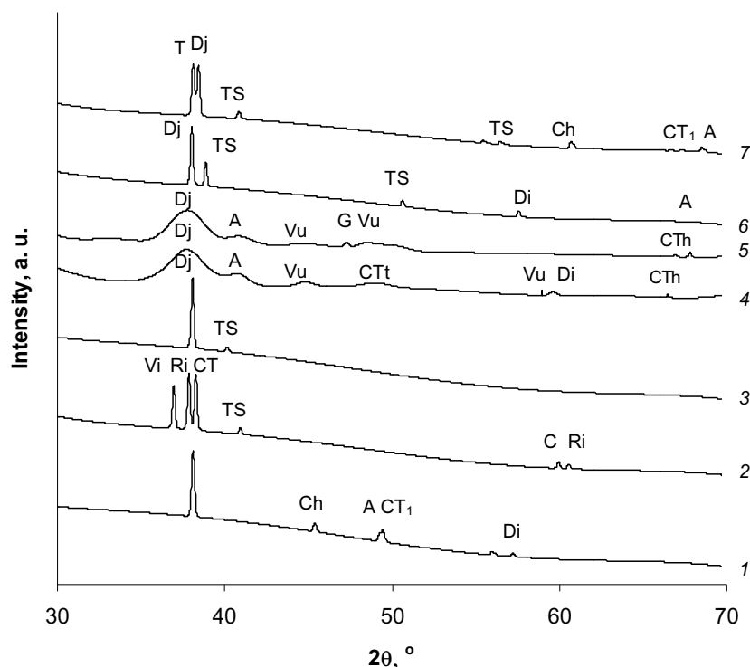
Fig. 6. XRD spectra of PA films first treated with the solutions of telluropentathionates at 20 °C and then with Cu(II/I) salts solution. PA chalcogenization precursor, duration of chalcogenization and concentration of its solution, mol/dm 3 : 1 – K 2 TeS 4 O 6 , 8 h, 0.025; 2 – K 2 TeS 4 O 6 , 8 h, 0.05; 3 – K 2 TeS 4 O 6 , 8 h, 0.1; 4 – Na 2 TeS 4 O 6 , 3 h, 0.05; 5 – Na 2 TeS 4 O 6 , 3 h, 0.1; 6 – H 2 TeS 4 O 6 , 5 h, 0.05; 7 – H 2 TeS 4 O 6 , 24 h, 0.05. A – anilite , Cu 7 S 4 ; Dj – djurleite , Cu 1.9375 S; Di – digenite , Cu 1.8 S; G – geerite , Cu 1.6 S; Ch – chalcocite , Cu 2 S; Vi – villamanite , CuS 2 ; C – covellite , CuS; CT – Cu 4 Te 3 ; CT 1 – Cu 1.85 Te; TS – tellurium sulfide, TeS 7 ; CTh – hexagonal copper telluride Cu 2 Te; CTt – tetragonal copper telluride Cu 3.18 Te 2 ; Vu – vulcanite , CuTe; Ri – rickardite , Cu 7 Te 5 ; T – tellurium
